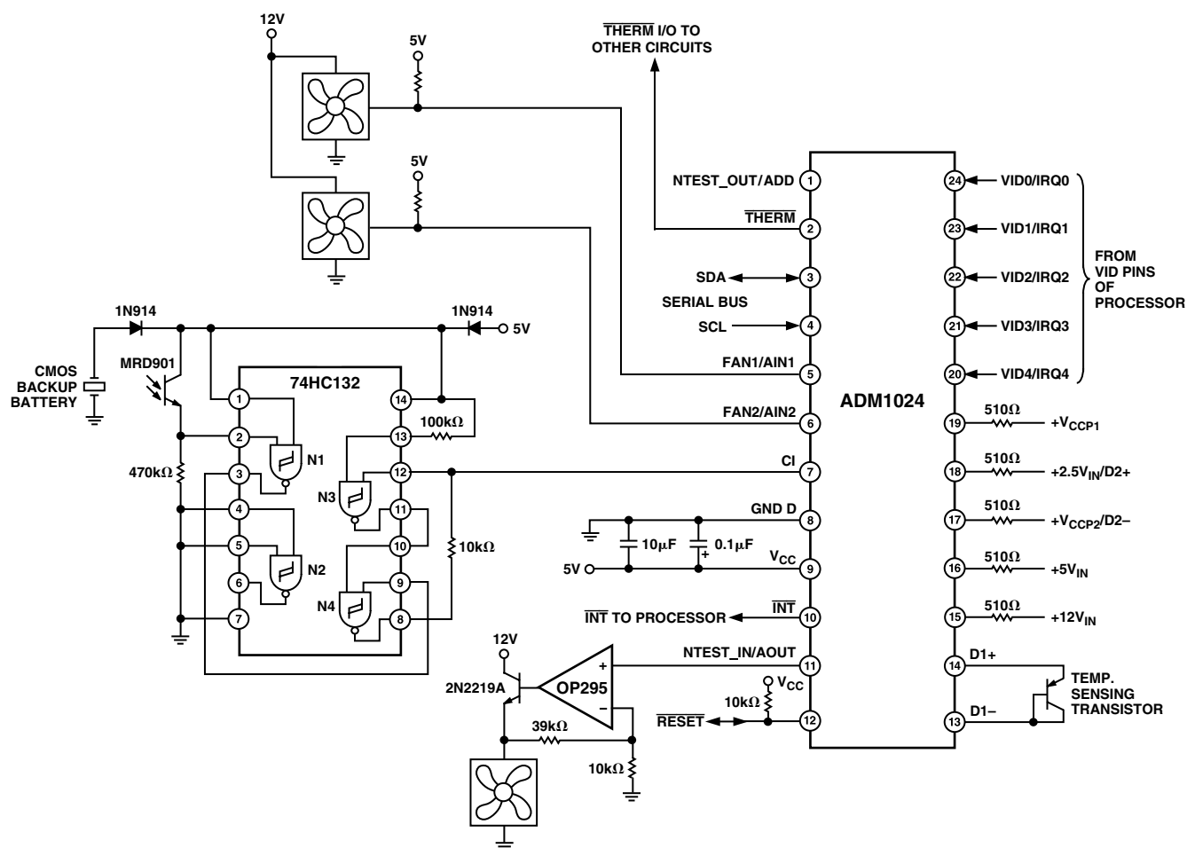
Figure 18. Application Circuit
