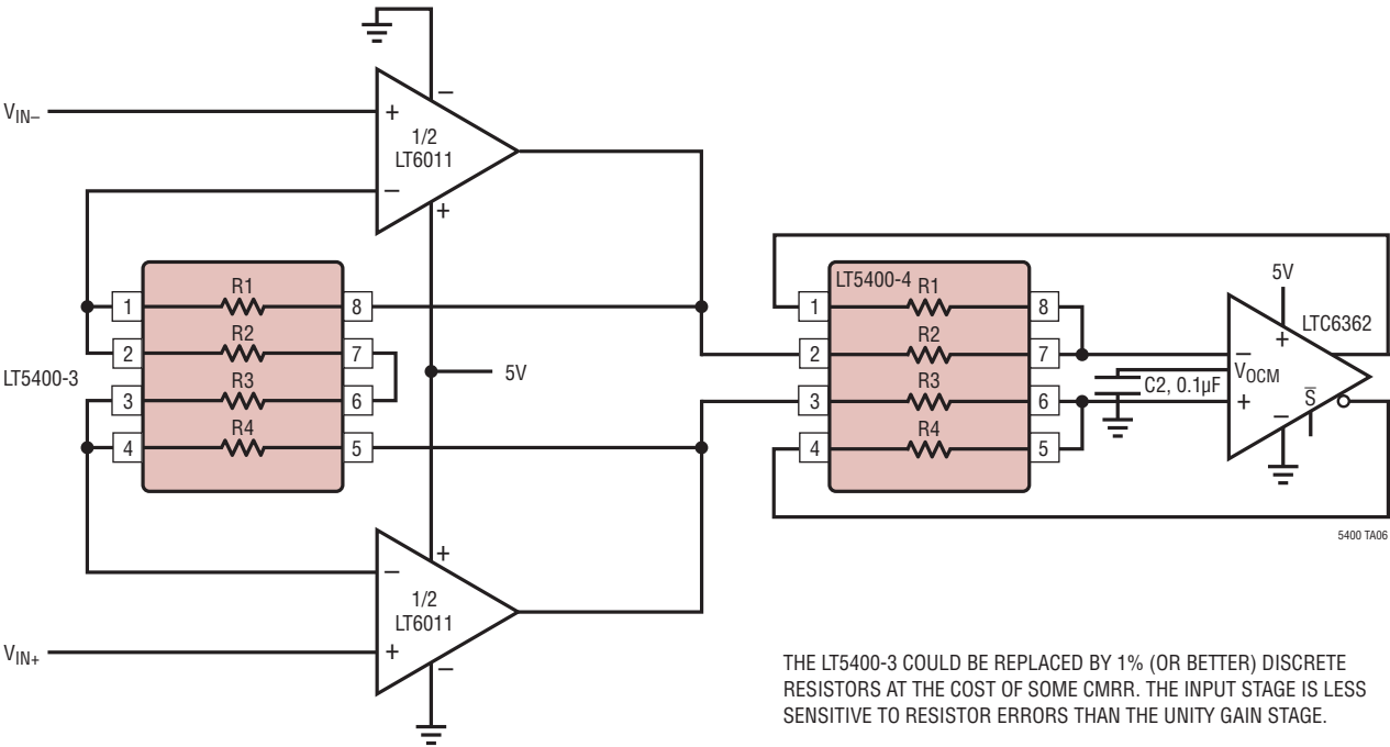
Gain of 10, 106dB CMRR, Discrete Component, Fully-Differential Instrumentation Amplifier
