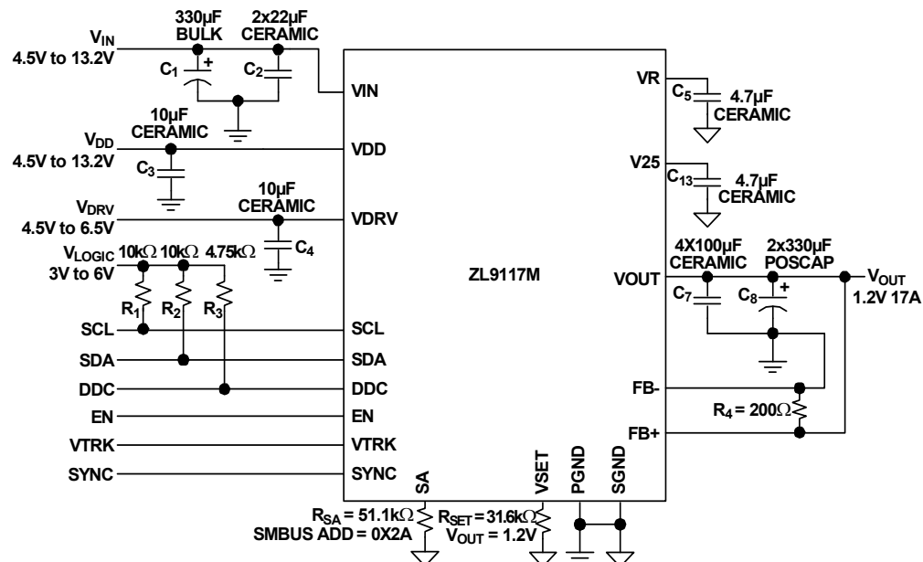
FIGURE 3. TYPICAL APPLICATION
