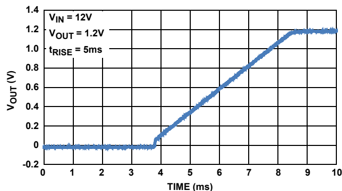
FIGURE 9. SOFT-START RAMP-UP
