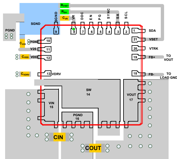
FIGURE 21. RECOMMENDED LAYOUT
