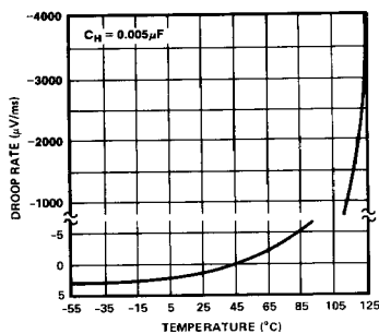
SMP-10 DROOP RATE vs TEMPERATURE
