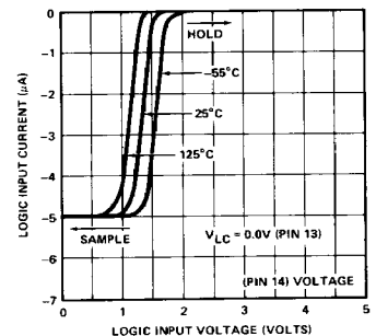
LOGIC INPUT CURRENT
