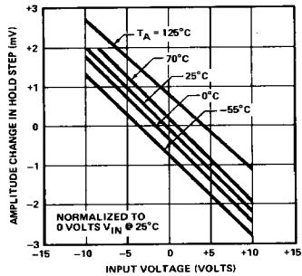
AMPLITUDE CHANGE IN HOLD STEP vs INPUT VOLTAGE
