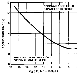
ACQUISITION TIME vs HOLD CAPACITOR
