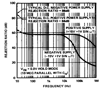
HOLD MODE POWER SUPPLY REJECTION
