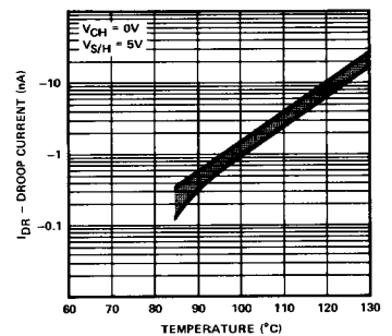
DROOP CURRENT vs TEMPERATURE
