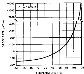
SMP-11 DROOP RATE vs TEMPERATURE
