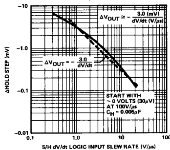
CHANGE IN HOLD STEP vs S/H \frac{dV}{dt}
