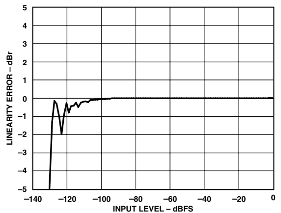
TPC 42. Linearity Error, 192 kHz:44.1 kHz, 0 dBFS to -140 dBFS Input, 200 Hz Tone
