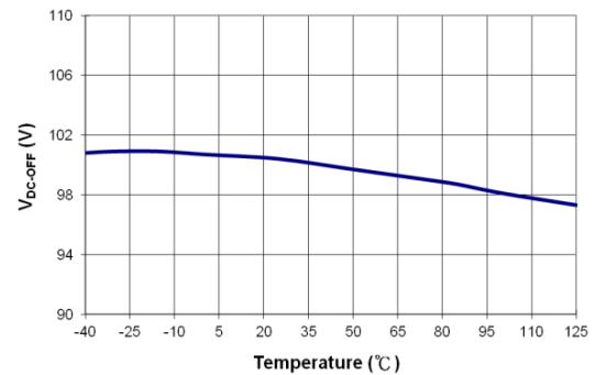
Figure 11. V_{DC-OFF} vs. Temperature
