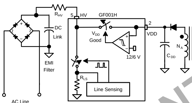
Figure 18. Functional Description
