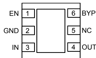
MIC5247-x.xBML / YML 6-Pin 2mm × 2mm MLF™ (ML) (Top View)
