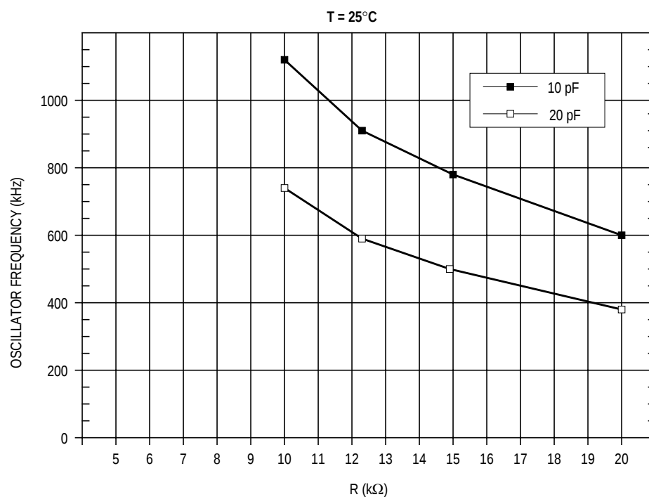
Figure 12-14. 3-Pin Oscillator R versus Frequency (V DD = 3.0 V)
