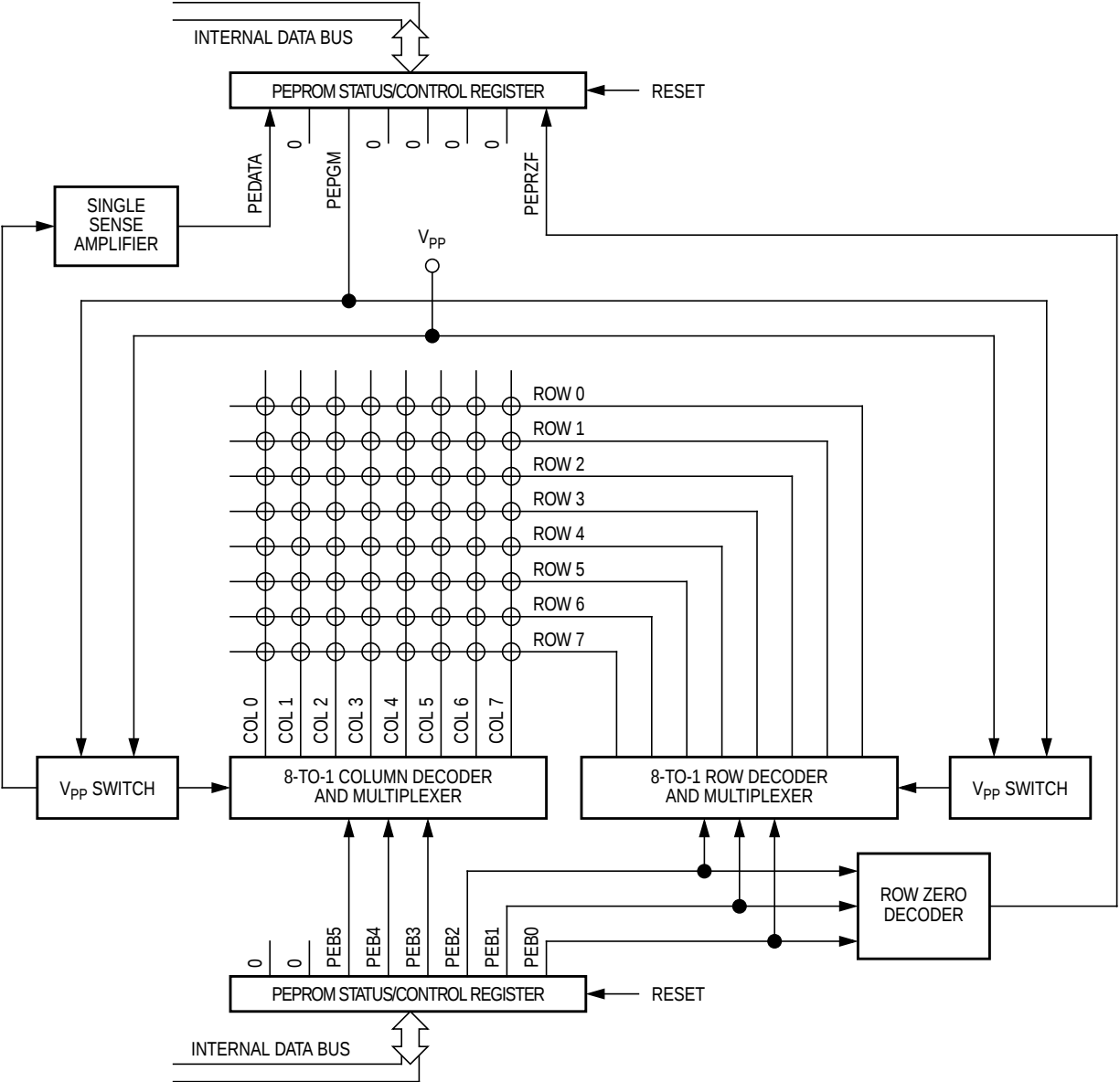
Figure 10-1. Personality EPROM
