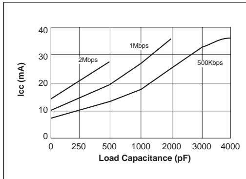
Figure 6. Icc VS. Load Capacitance for the SP3220EU.
