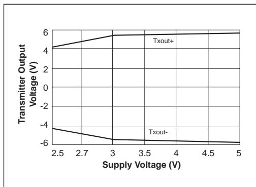
Figure 8. Transmitter Output Voltage VS. Supply Voltage for the SP3220EU.
