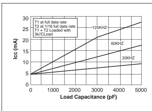
Figure 1. I_{cc} VS. Load Capacitance for the SP3220EB.
