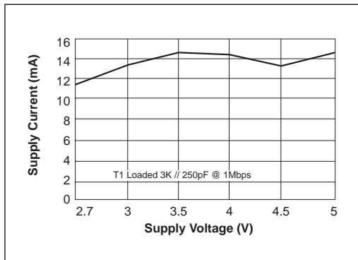
Figure 9. Supply Current VS. Supply Voltage for the SP3220EU.
