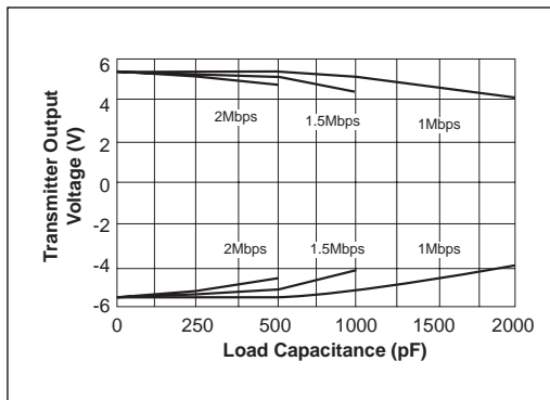
Figure 7. Transmitter Output Voltage VS. Load Capacitance for the SP3220EU.
