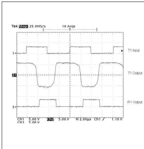
Figure 13. SP3220EB Driver Loopback Test Results at 250Kbps.
