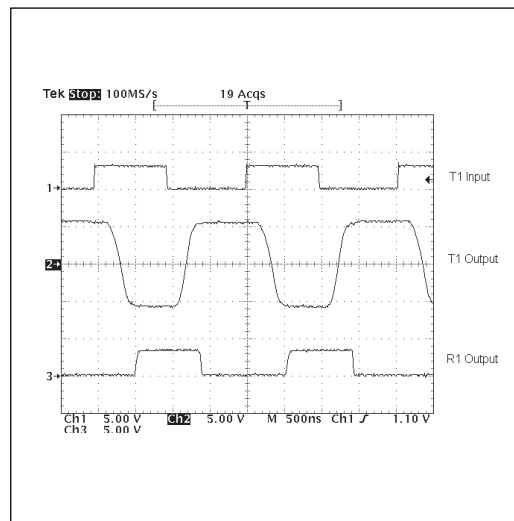
Figure 14. SP3220EU Driver Loopback Test Results at 1Mbps.
