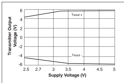
Figure 3. Transmitter Output Voltage VS. Supply Voltage for the SP3220EB.
