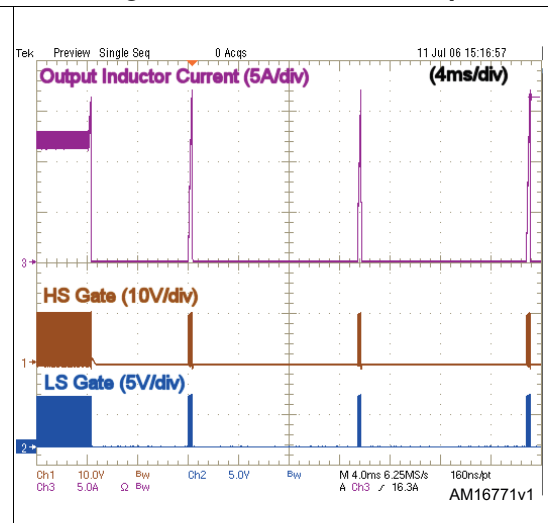
Figure 7. Overcurrent hiccup
