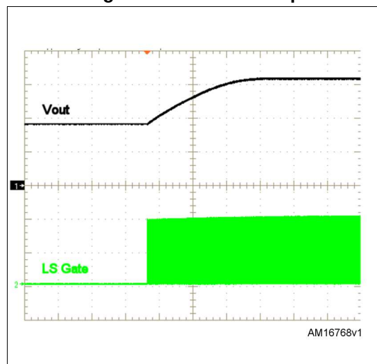
Figure 4. LS-less startup
