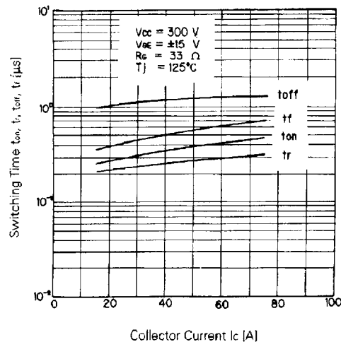
Switching Time
