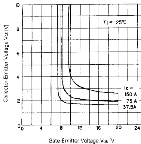
Collector-Emitter Voltage vs. Gate-Emitter Voltage
