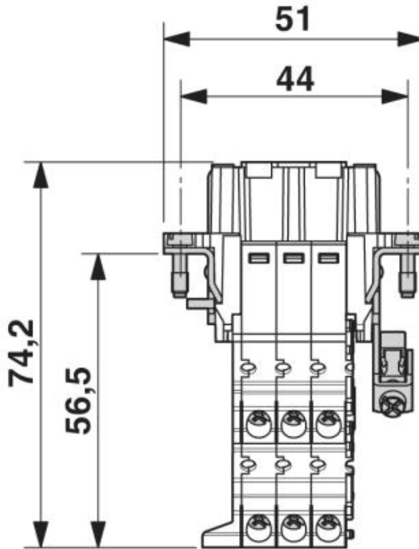
Dimensional drawing
