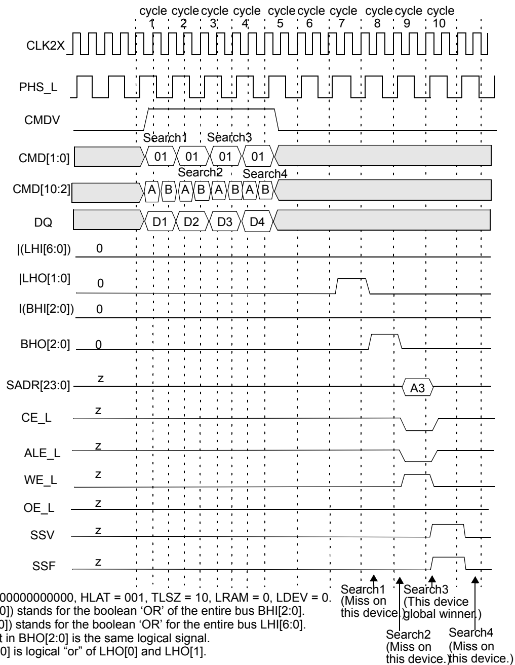
Figure 10-14. Timing Diagram for Globally Winning Device in Block Number 1
