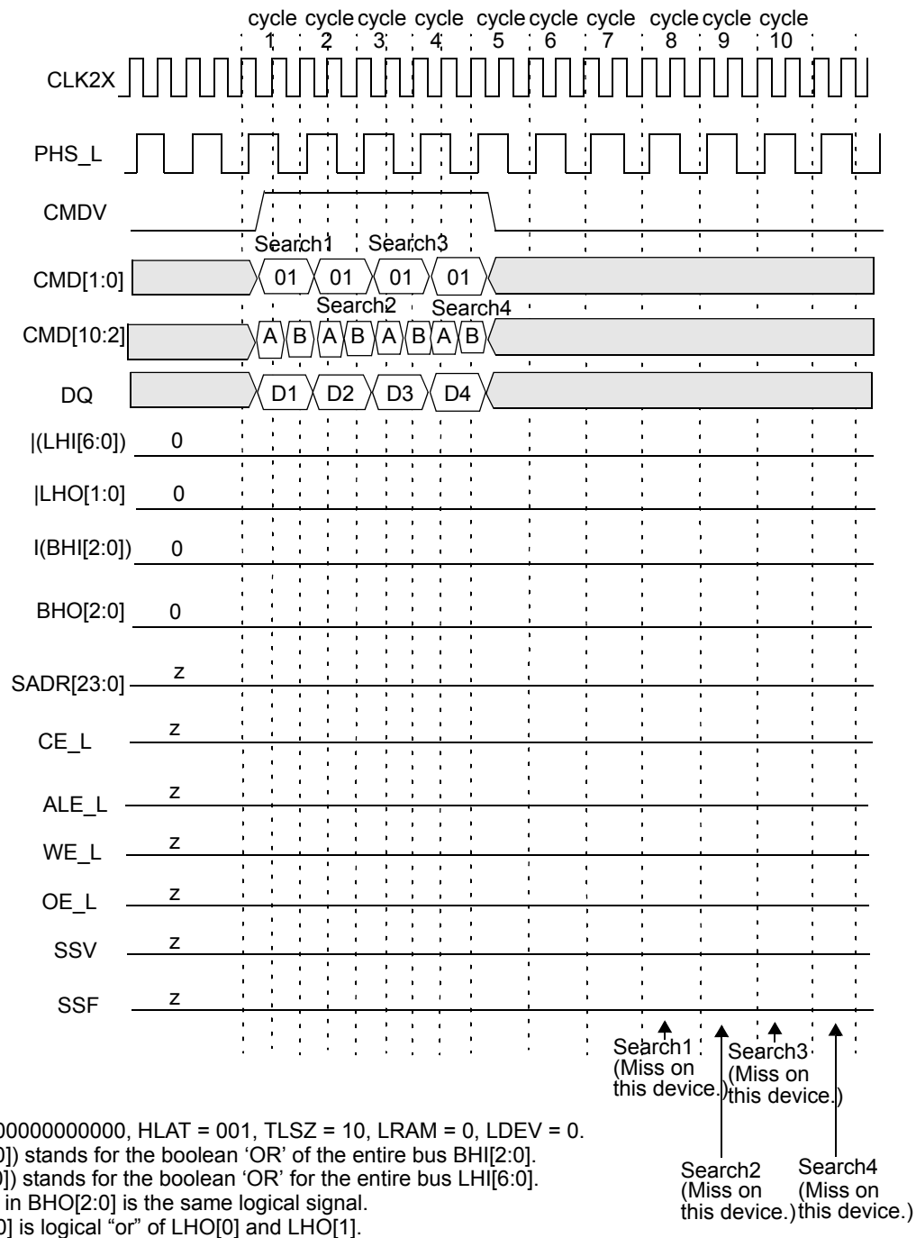
Figure 10-13. Timing Diagram for Each Device Above the Winning Device in Block Number 1
