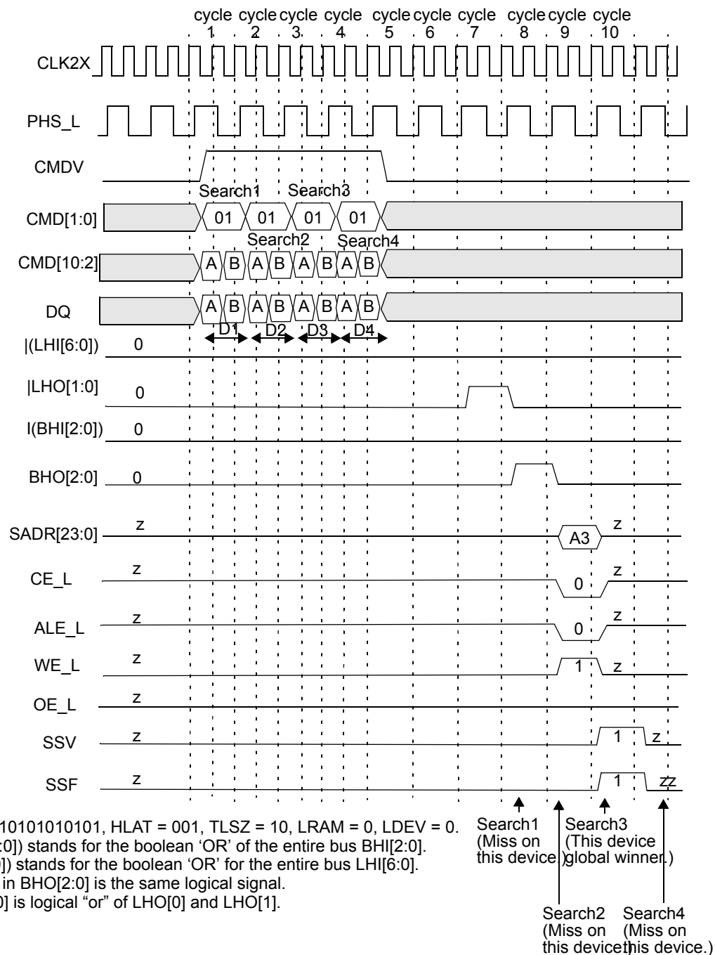
Figure 10-33. Timing Diagram for Globally Winning Device in Block Number 1
