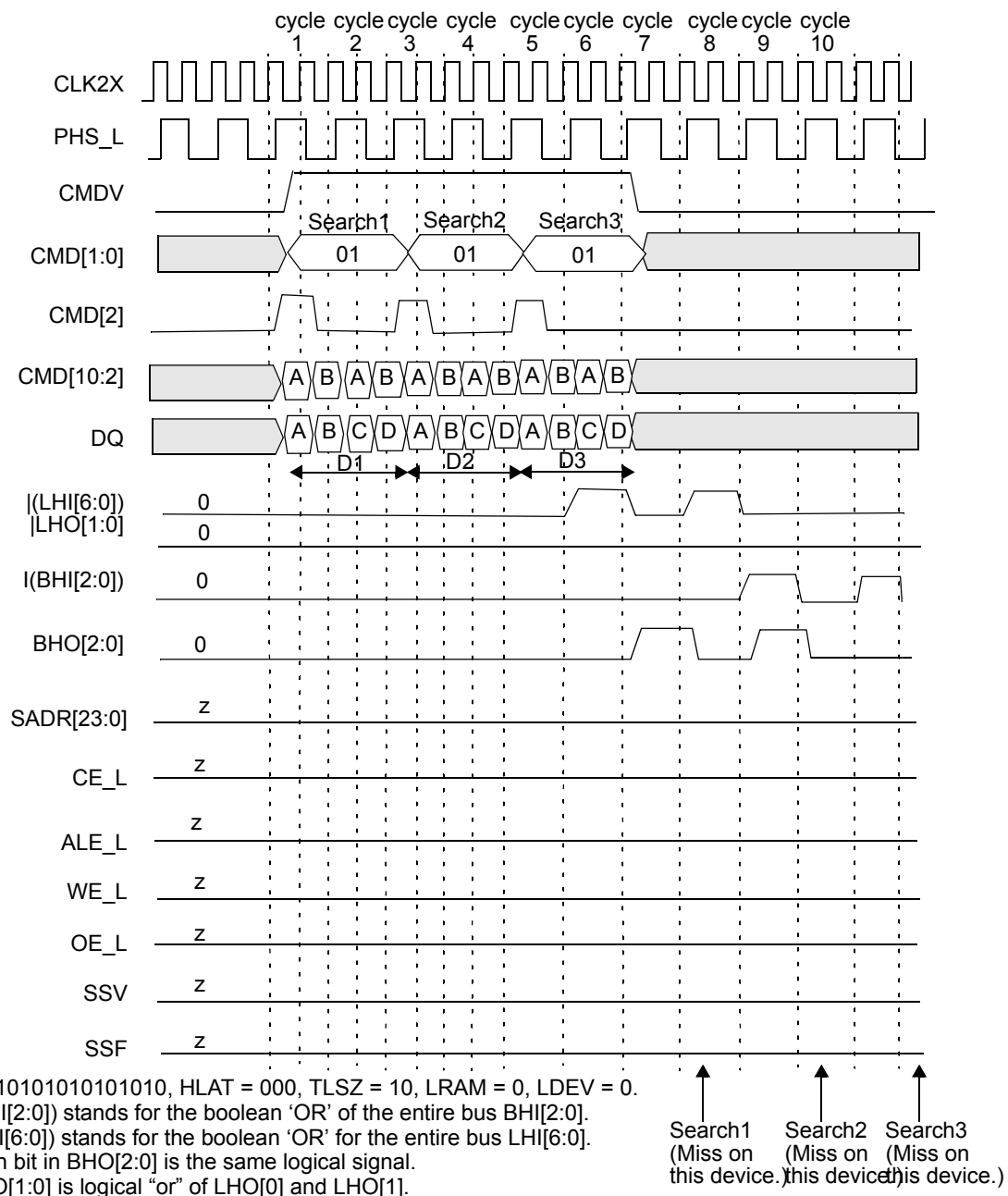
Figure 10-59. Timing Diagram for Devices Below the Winning Device in Block Number 3 Except Device 14 (Last Device)
