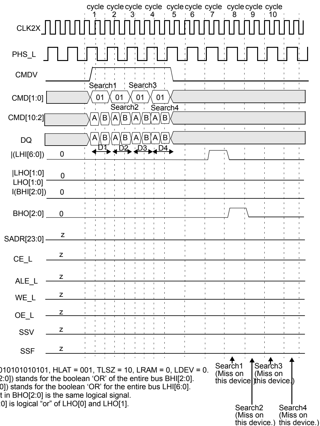
Figure 10-34. Timing Diagram for Devices Below the Winning Device in Block Number 1
