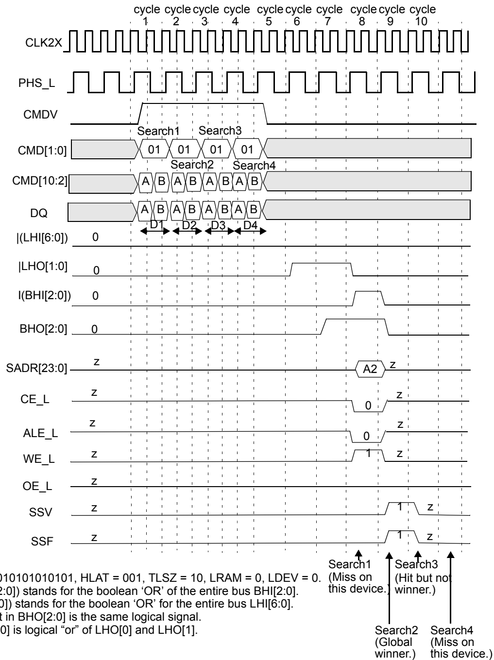
Figure 10-36. Timing Diagram for Globally Winning Device in Block Number 2
