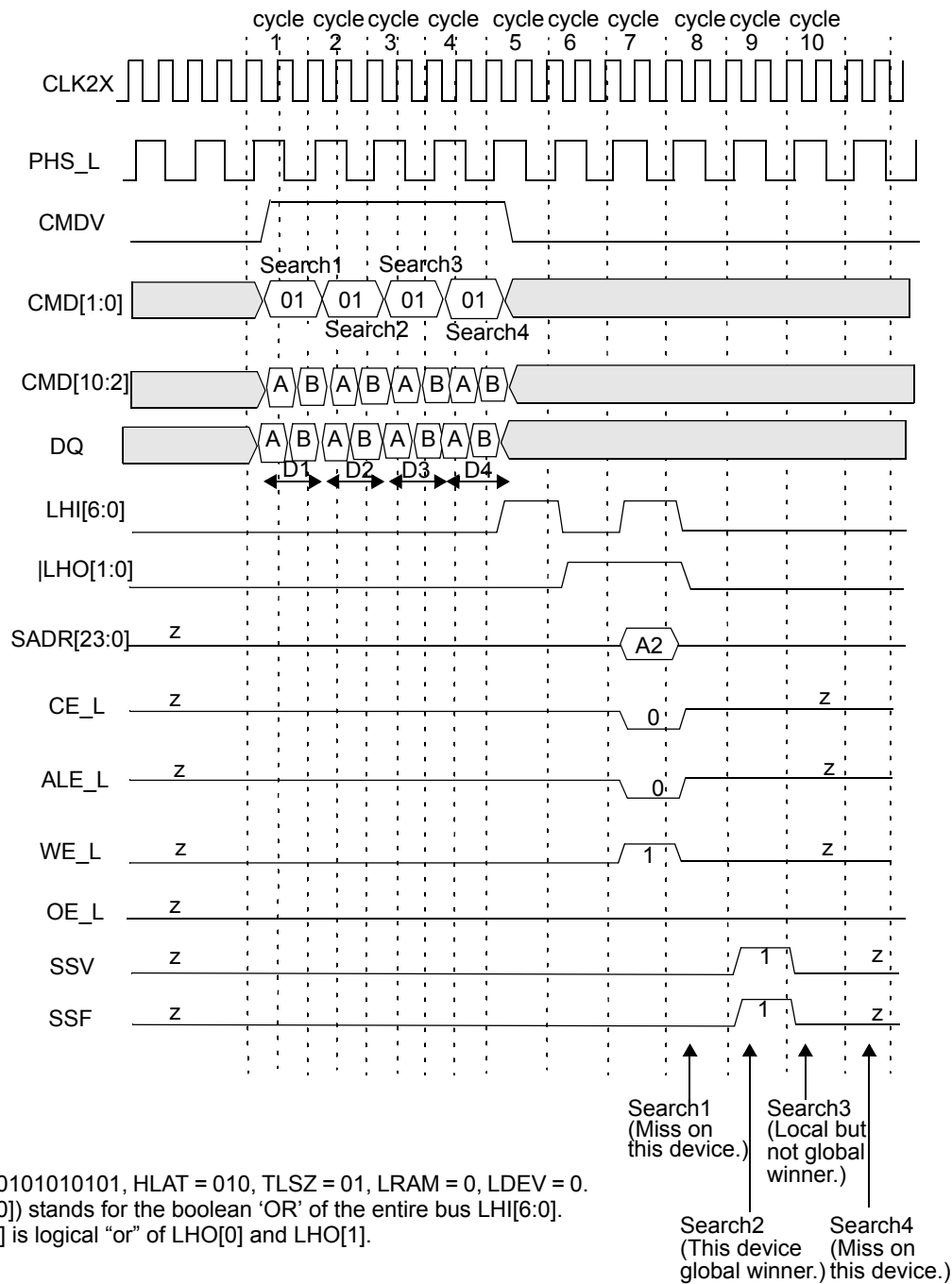
Figure 10-26. Timing Diagram for 144-bit Search Device Number 1
