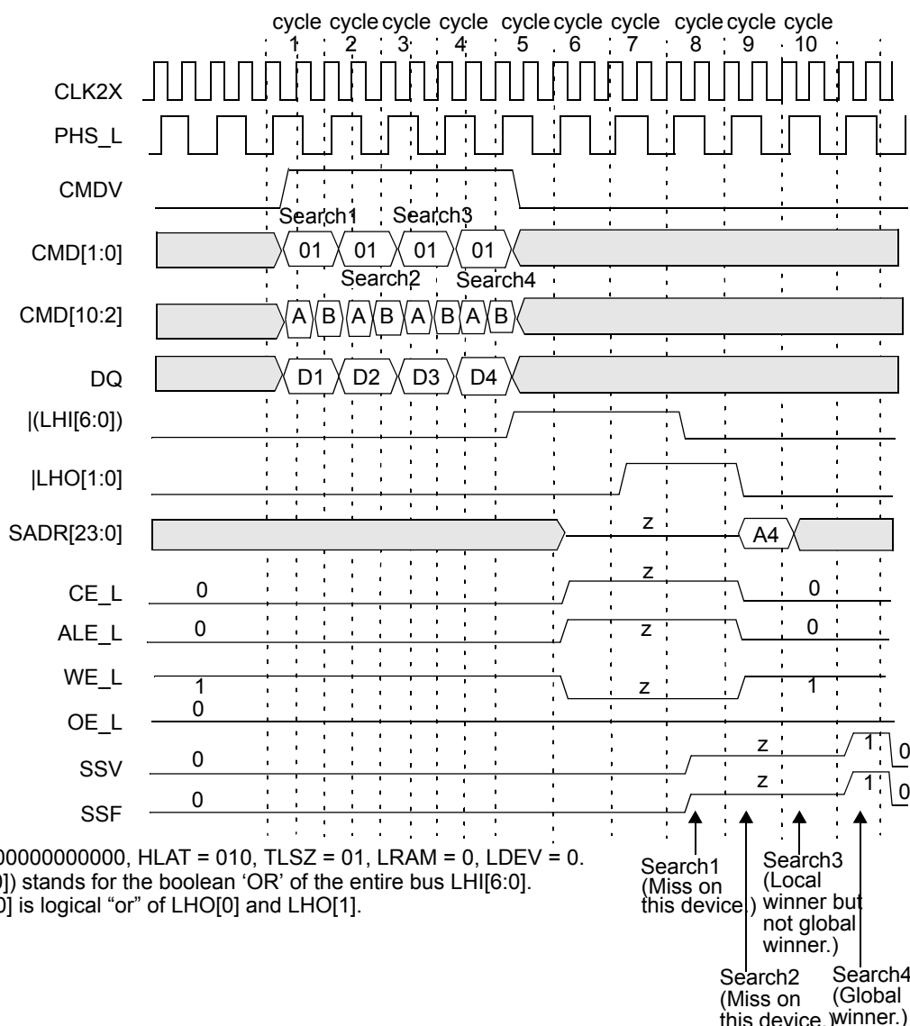
Figure 10-8. Timing Diagram for 72-bit Search Device Number 3 (Last Device)
