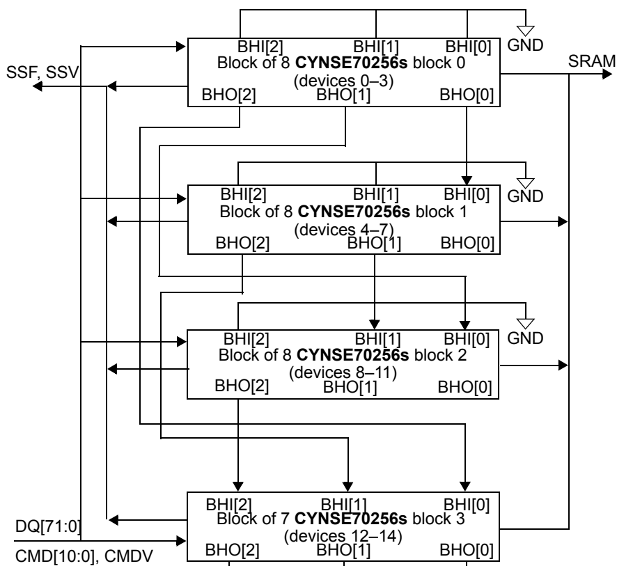
Figure 10-48. Hardware Diagram for a Table with Fifteen Devices
