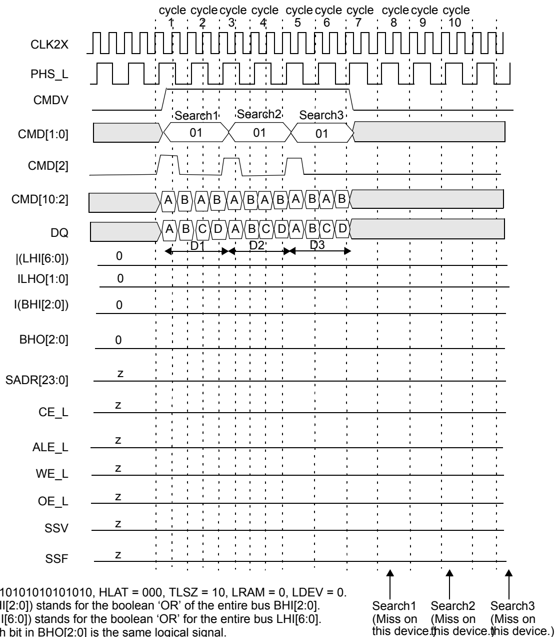
Figure 10-51. Timing Diagram for Each Device Above the Winning Device in Block Number 1
