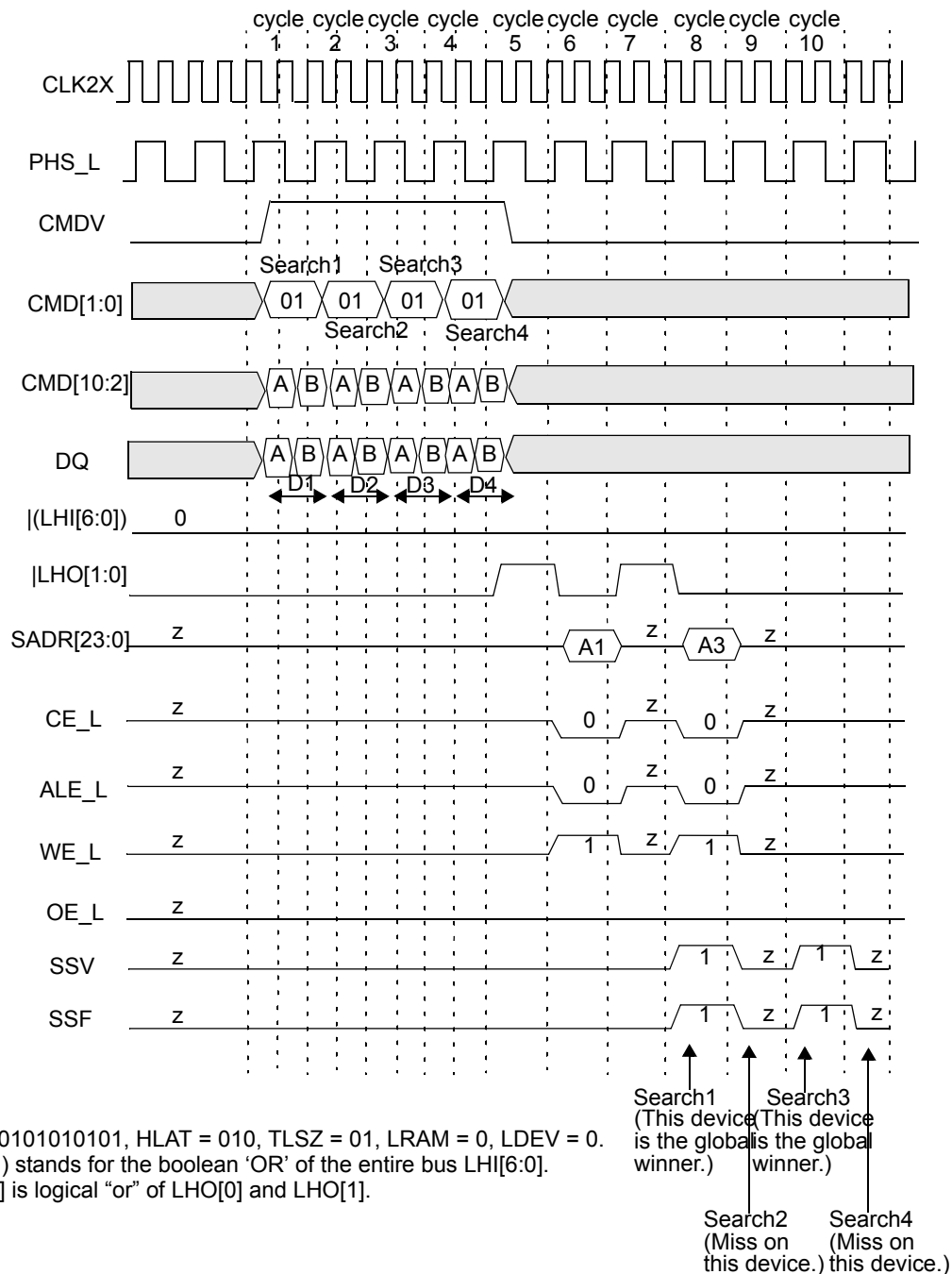
Figure 10-25. Timing Diagram for 144-bit Search Device Number 0
