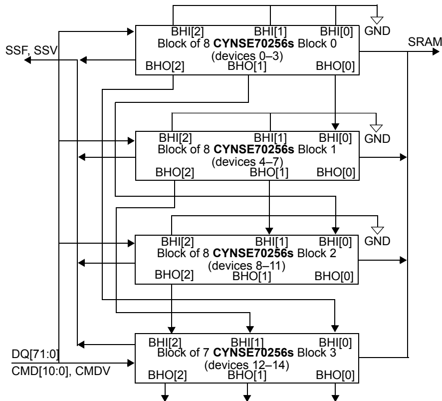
Figure 11-2. Depth Cascading four Blocks
