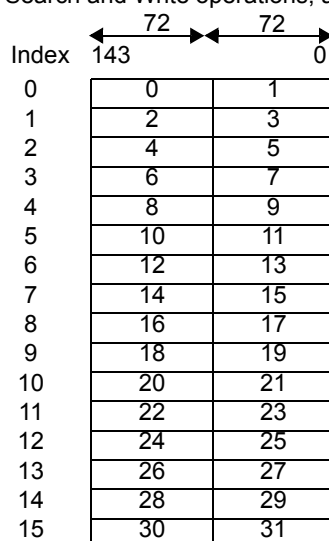
Figure 7-2. Addressing the GMR Array
