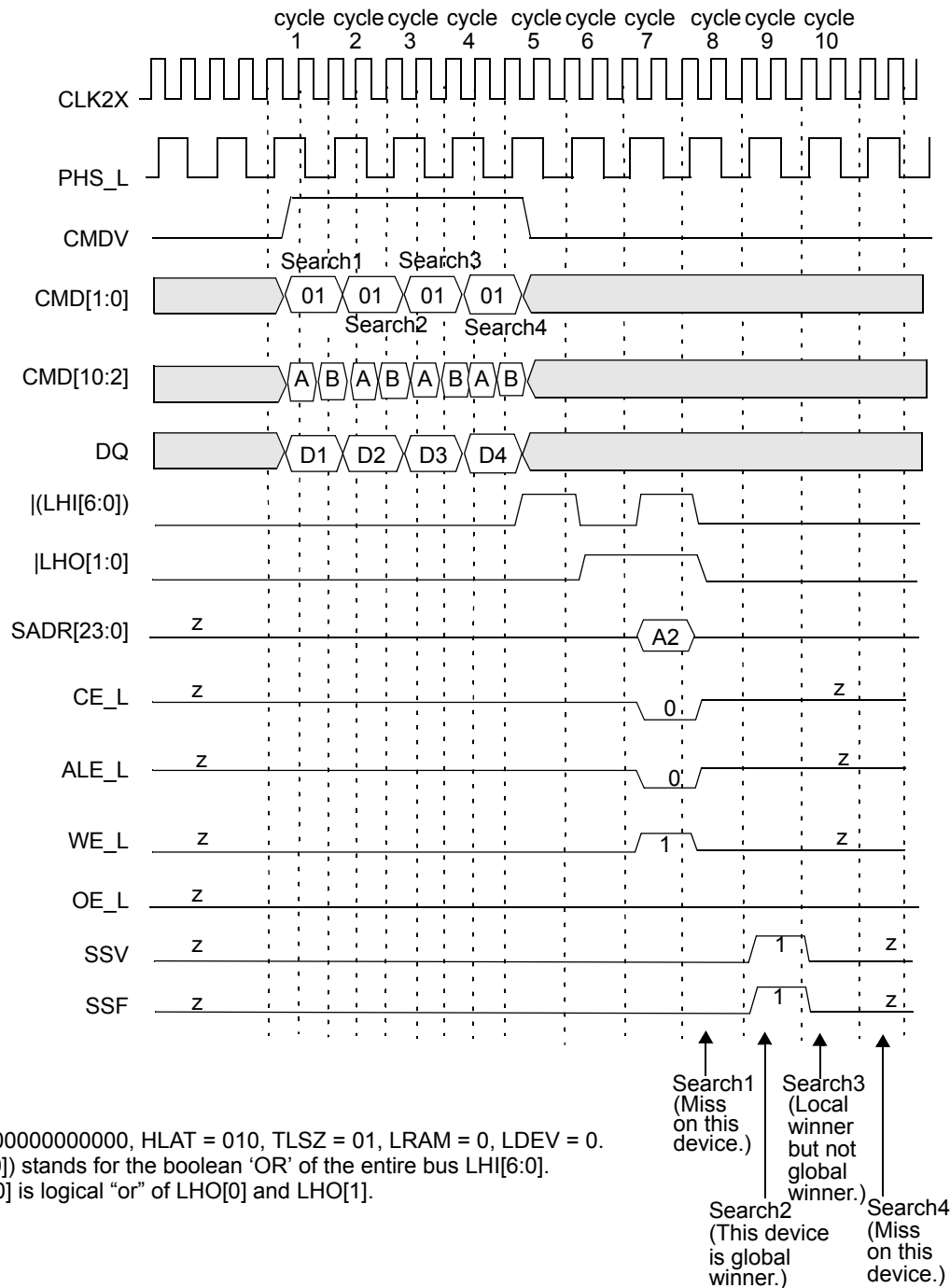
Figure 10-7. Timing Diagram for 72-bit Search Device Number 1
