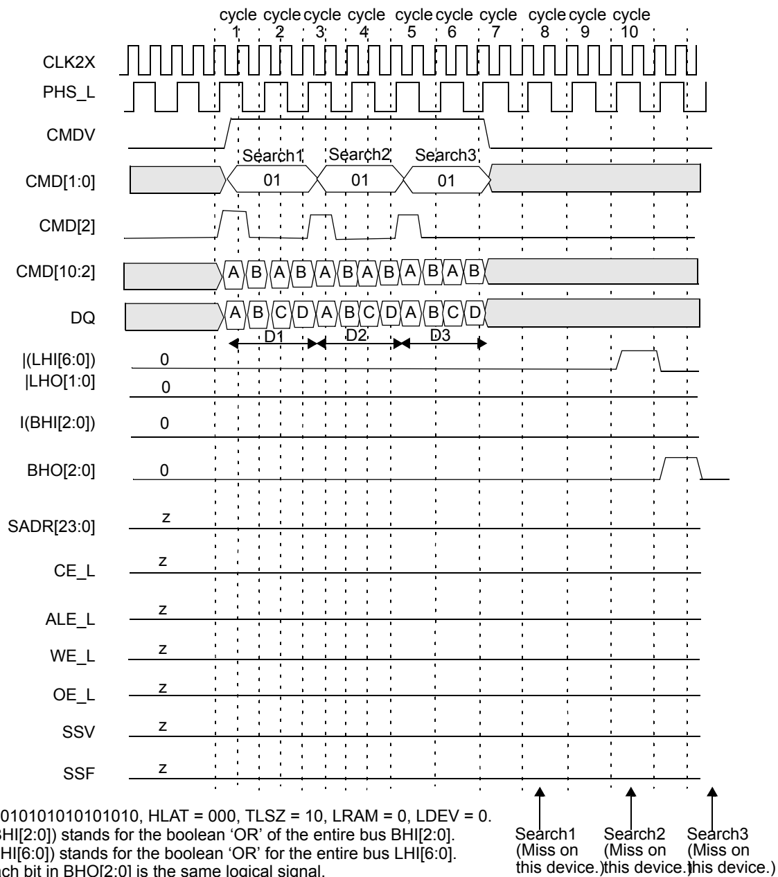
Figure 10-53. Timing Diagram for Devices Below the Winning Device in Block Number 1
