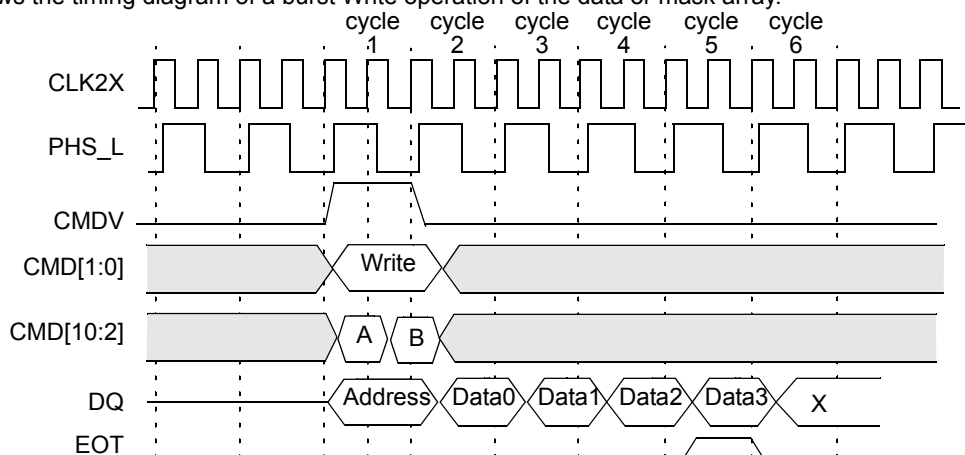
Figure 10-4. BURST Write of the Data and Mask Arrays (BLEN = 4)
