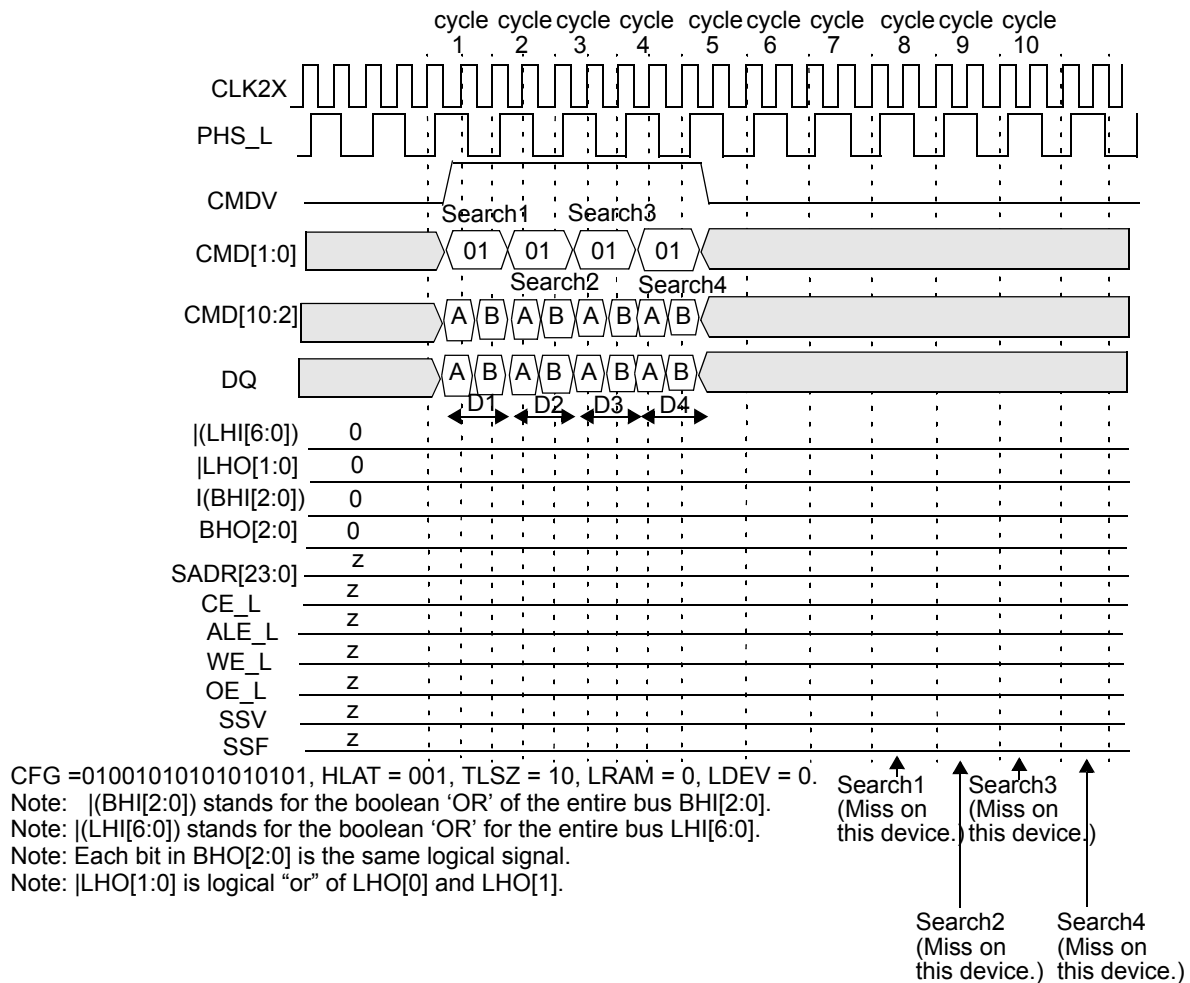
Figure 10-32. Timing Diagram for Each Device Above the Winning Device in Block Number 1
