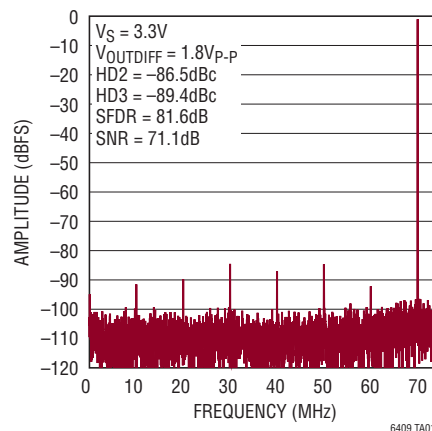
LTC6409 Driving LTC2262-14 ADC, f_{IN} = 70\text{MHz} , -1dBFS, f_s = 150\text{MHz} , 4096-Point FFT
