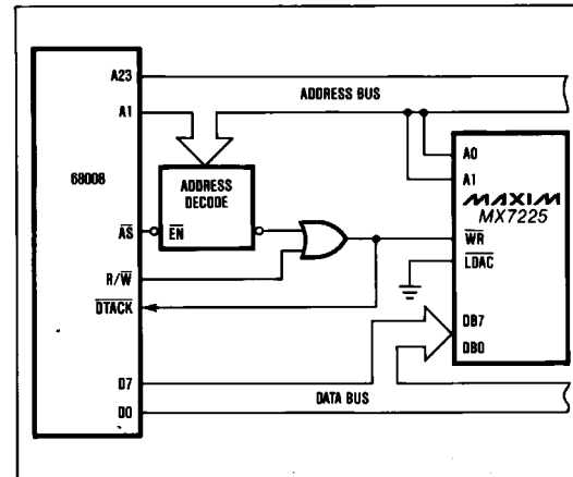
Figure 18. MX7225 to 68008 Interface, Single-Buffered Mode
