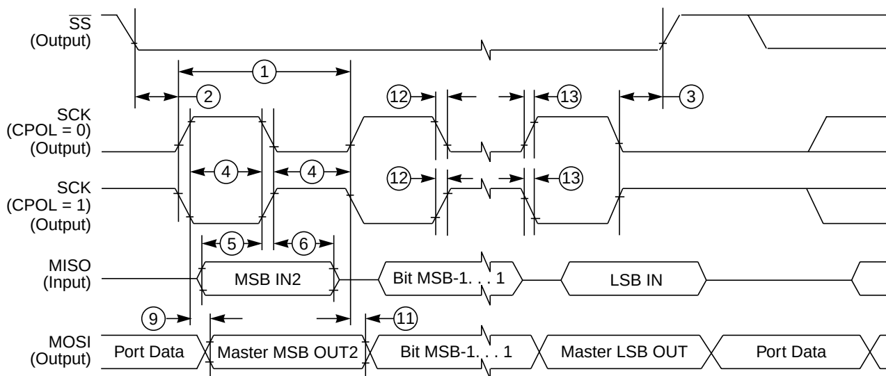
Figure A-9. SPI Master Timing (CPHA = 1)
