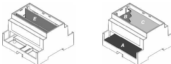
Horizontal PCB Positions
