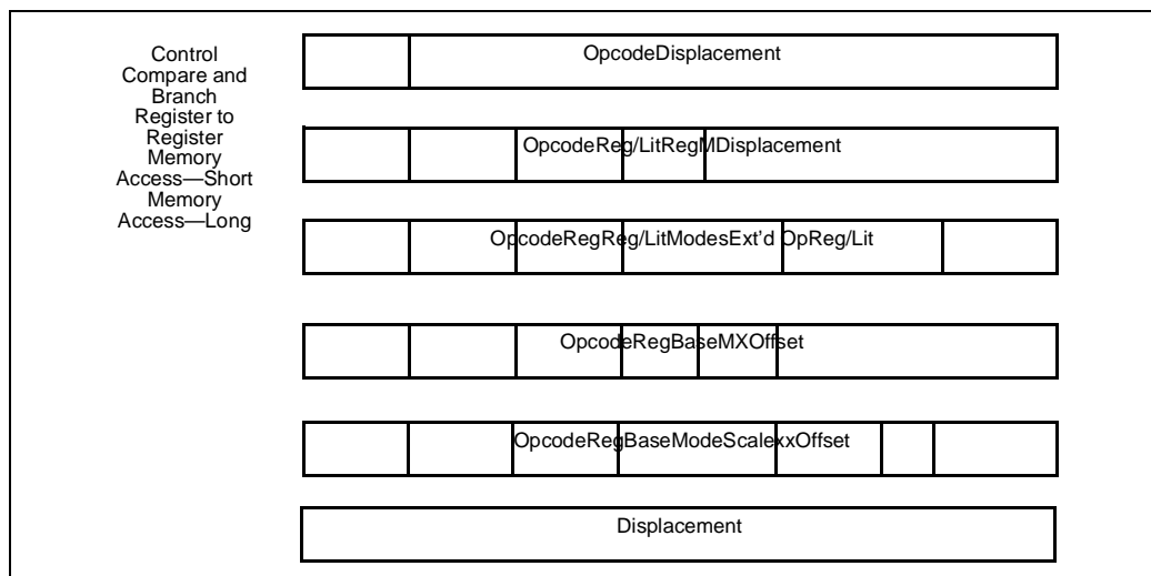
Figure 3. Instruction Formats
