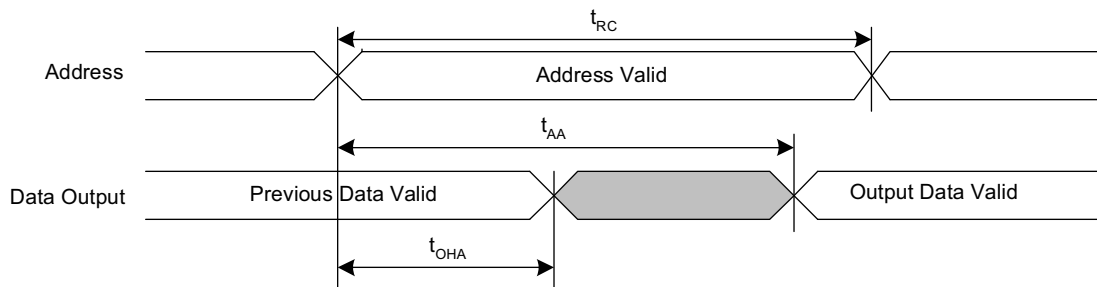
Figure 6. SRAM Read Cycle #1: Address Controlled [12, 13, 16]
