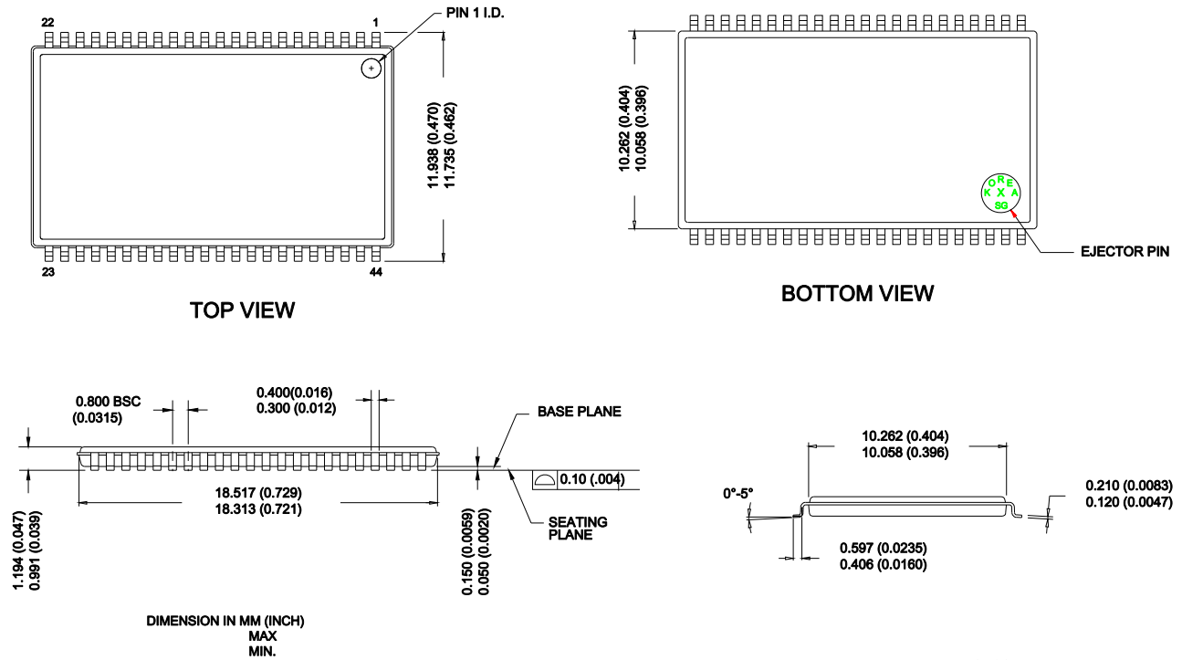
Figure 16. 44-Pin TSOP II
