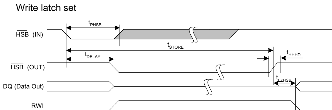
Figure 14. Hardware STORE Cycle [19]
