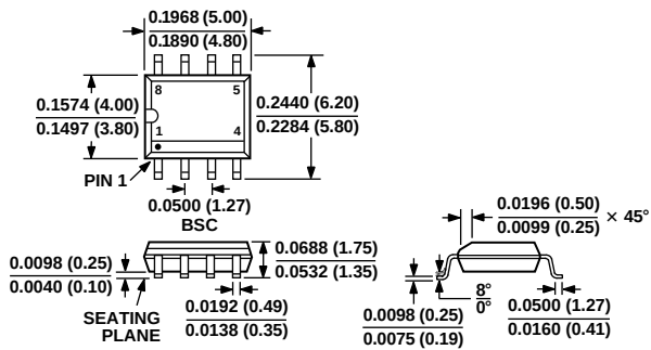
8-Lead Plastic SOIC (SO-8)
