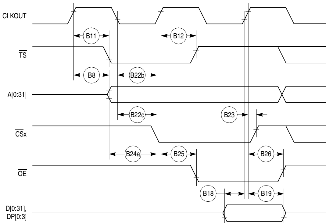
Figure 13. External Bus Read Timing (GPCM Controlled—TRLX = 0, ACS = 11)
