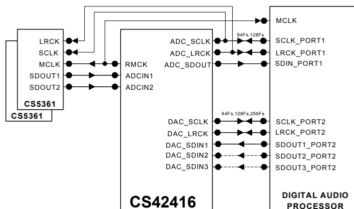
Figure 19. OLM Configuration #3
