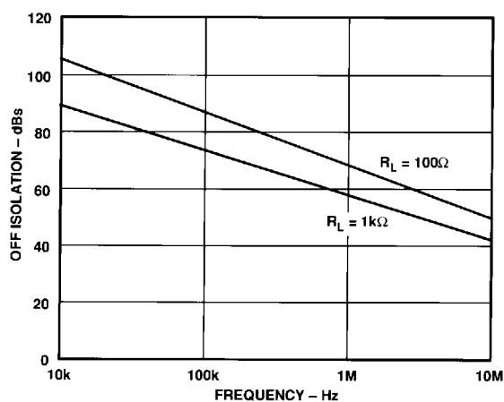
Off Isolation vs. Signal Frequency; Dual or Single 15V Supplies, T_A = +25^\circ C
