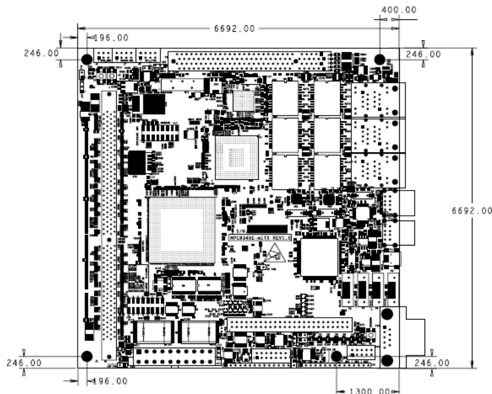
Figure 21. Dimensions of the MPC8349E-mITX-GP Board
