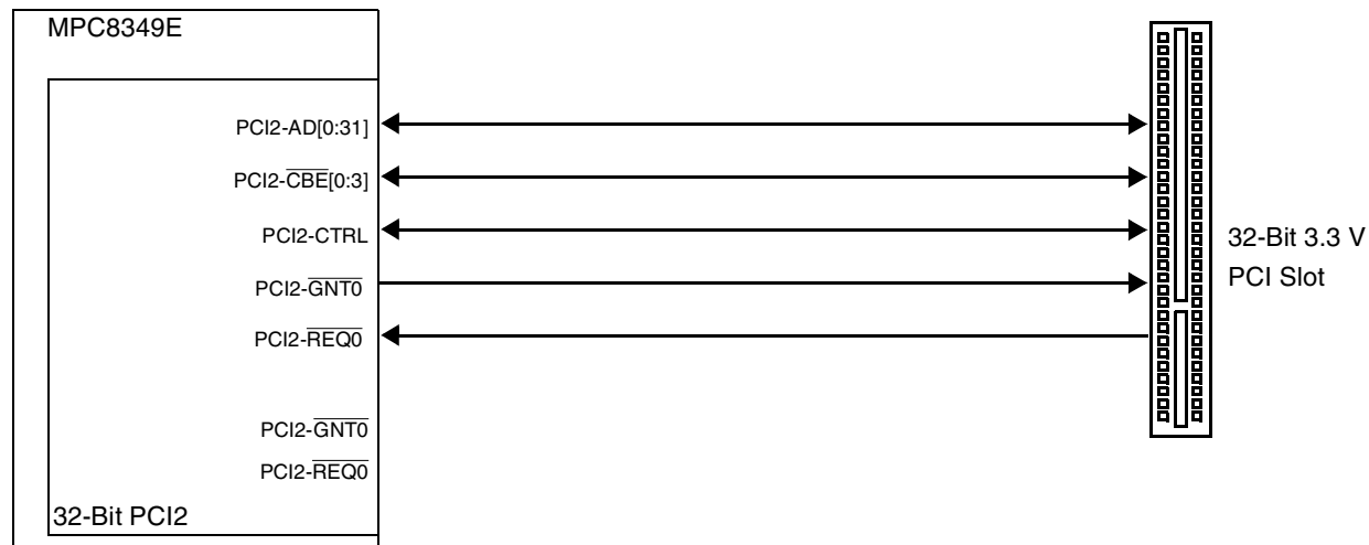
Figure 10. PCI Subsystem
