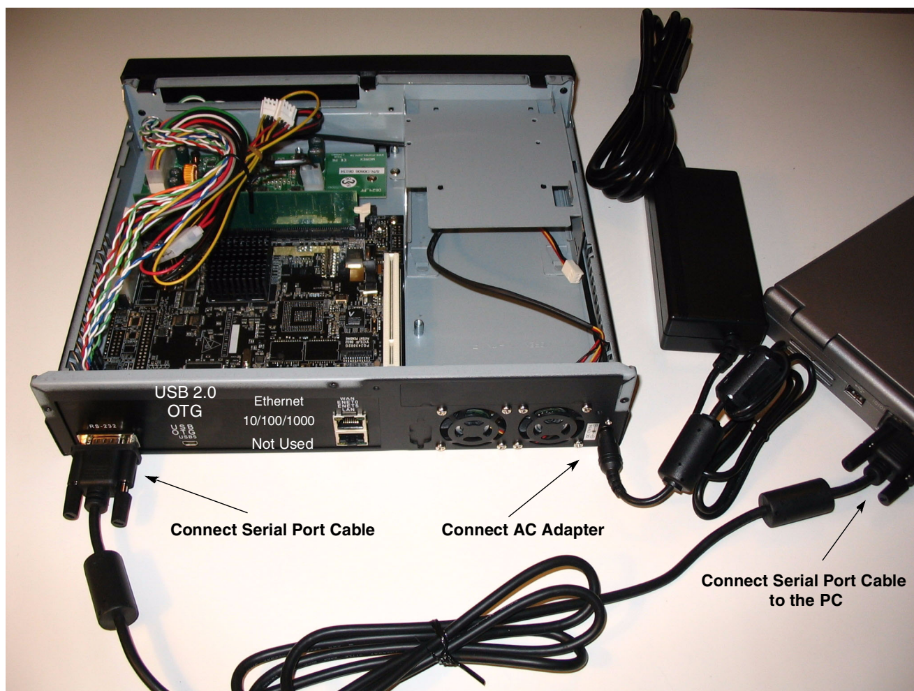
Figure 24. External Connections
