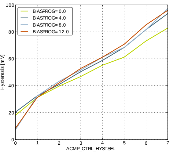
Hysteresis
