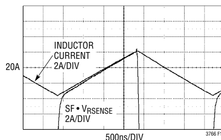
Figure 13. Properly Calibrated Current Transformer
