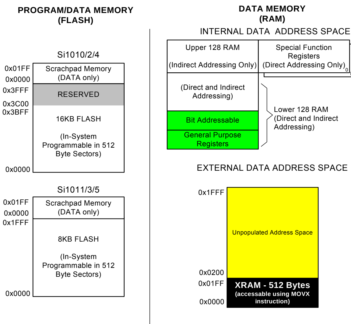
Figure 9.1. Si1010/1/2/3/4/5 Memory Map
