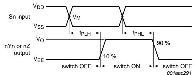
Fig 13. Sn to nYn, nZ propagation delays
