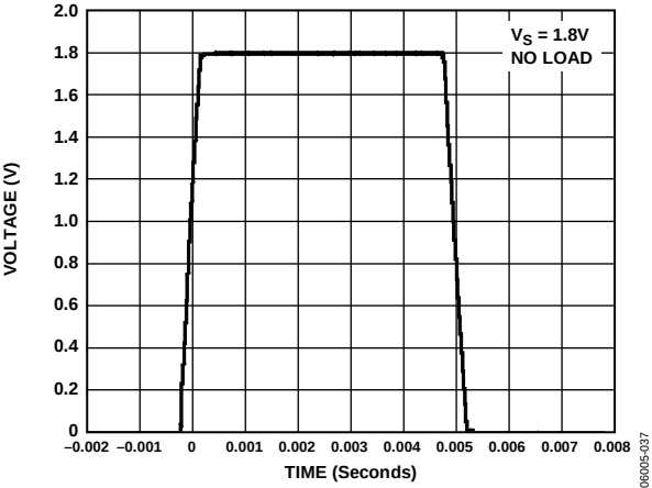
Figure 37. Large Signal Transient Response
