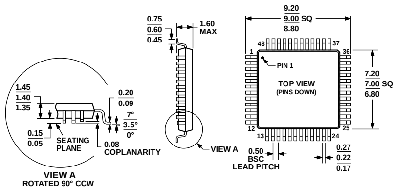
Figure 39. 48-Lead Low Profile Quad Flat Package [LQFP]
