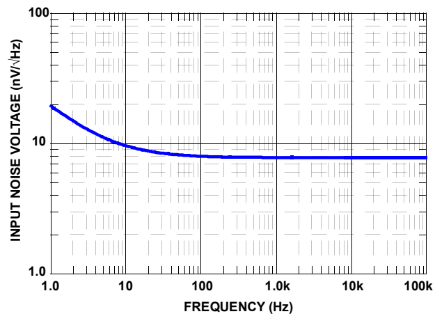
FIGURE 59. SIMULATED INPUT NOISE VOLTAGE
