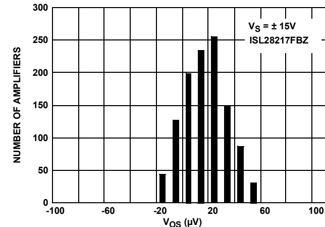
FIGURE 5. V_{OS} DISTRIBUTION FOR GRADE C
