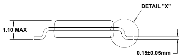
SIDE VIEW 2
