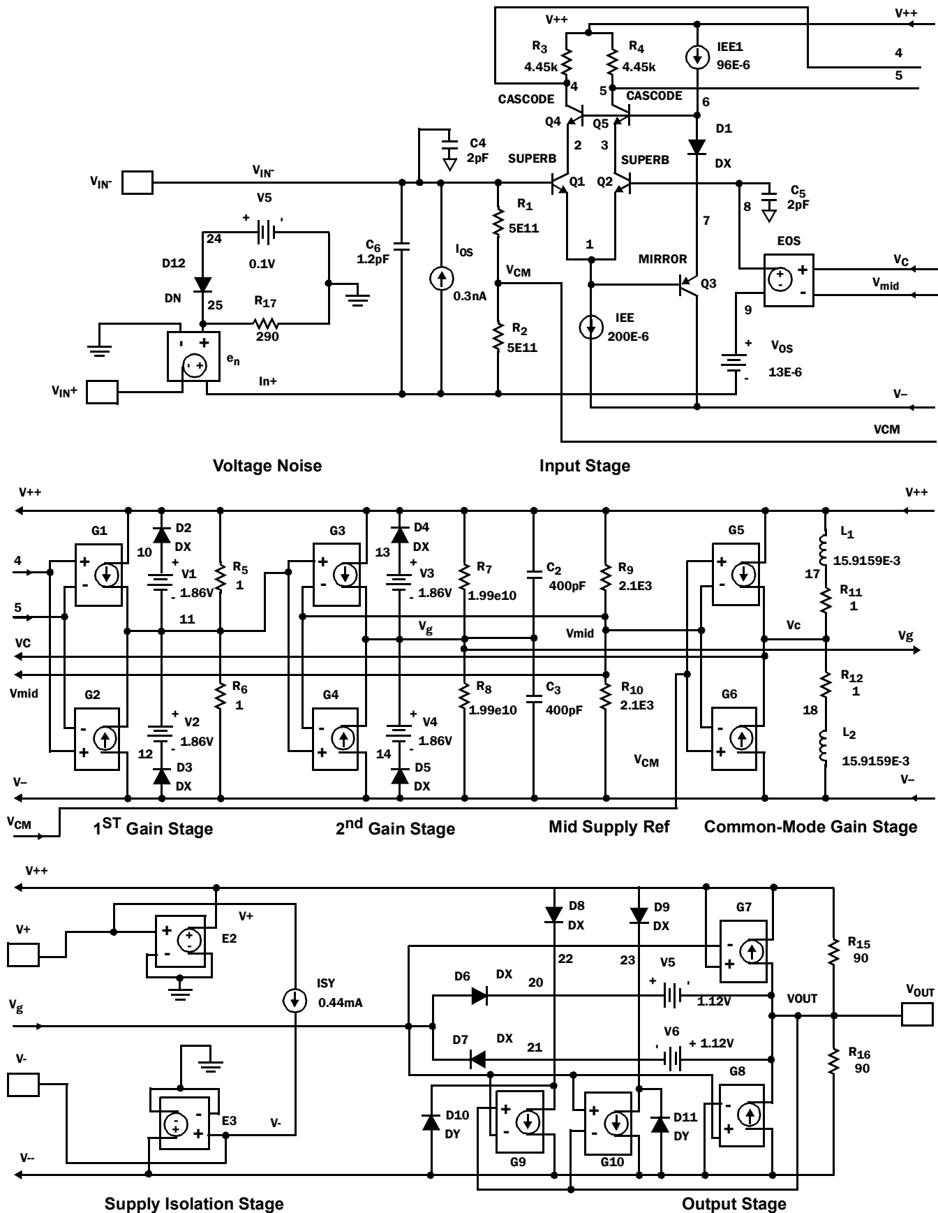
FIGURE 56. SPICE SCHEMATIC
