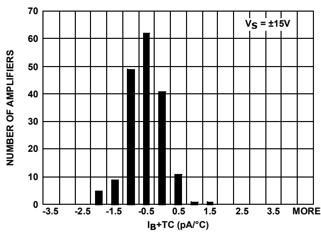
FIGURE 12. TCI_{B+} vs NUMBER OF AMPLIFIERS
