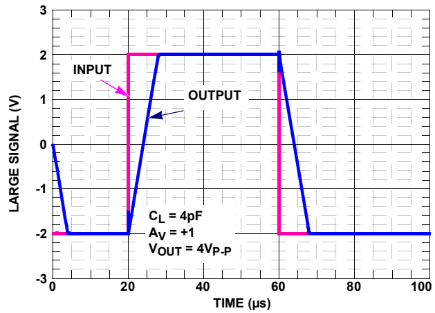
FIGURE 65. SIMULATED LARGE SIGNAL 10V STEP RESPONSE
