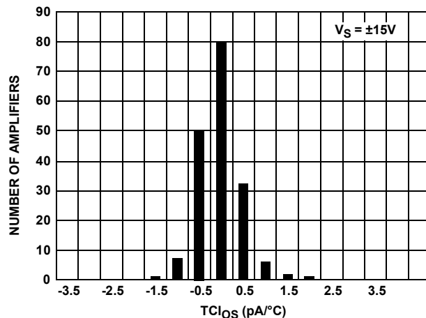
FIGURE 20. I_{OS}TC vs NUMBER OF AMPLIFIERS
