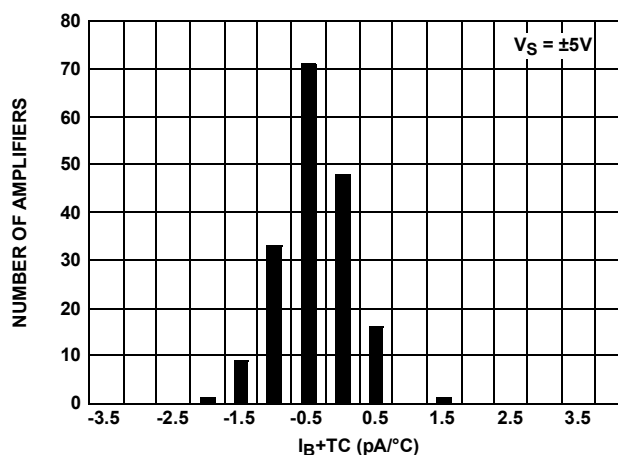
FIGURE 16. TCI_{B+} vs NUMBER OF AMPLIFIERS
