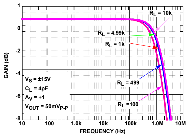
FIGURE 63. SIMULATED CLOSED LOOP GAIN vs R_L
