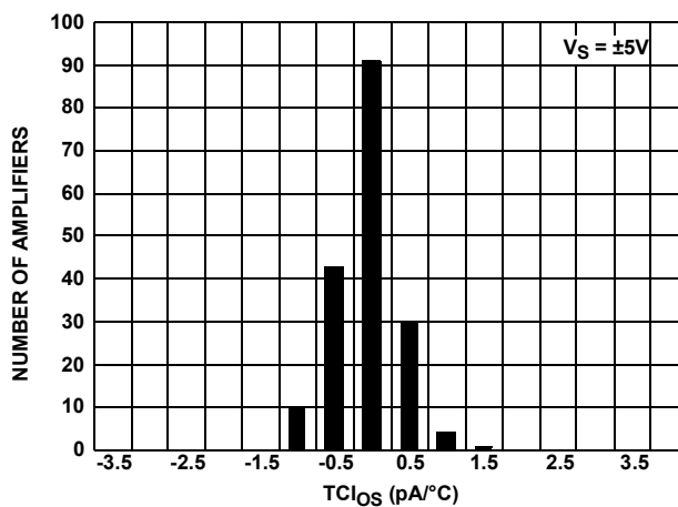
FIGURE 22. I_{OS}TC vs NUMBER OF AMPLIFIERS
