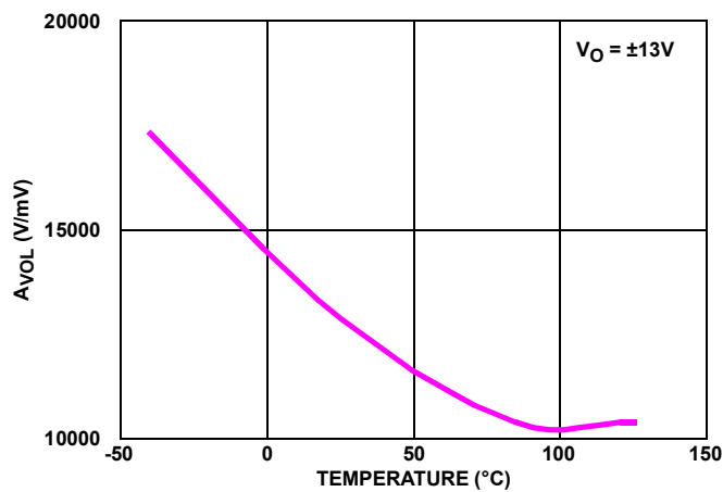
FIGURE 24. A_{VOL} vs TEMPERATURE
