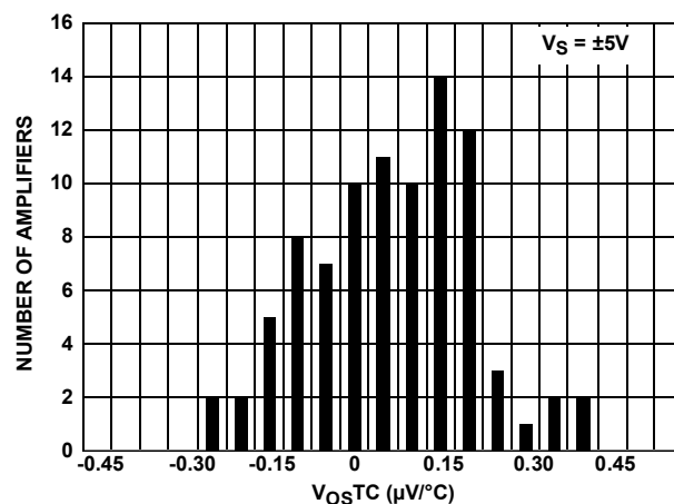
FIGURE 10. TCV_{OS} vs NUMBER OF AMPLIFIERS
