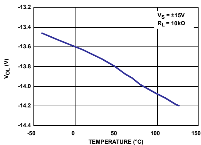
FIGURE 32. V_{OL} vs TEMPERATURE,
