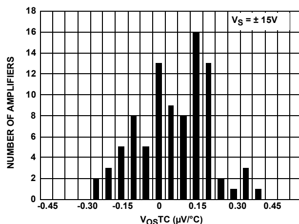
FIGURE 8. TCV_{OS} vs NUMBER OF AMPLIFIERS
