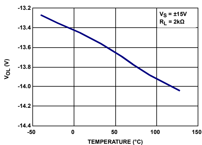
FIGURE 34. V_{OL} vs TEMPERATURE
