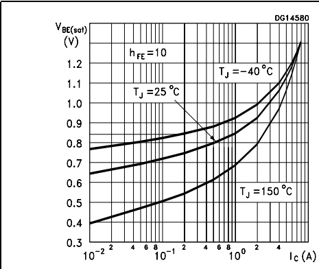
Figure 10. Base-emitter saturation voltage (NPN)
