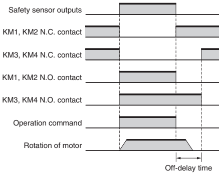
Timing chart
