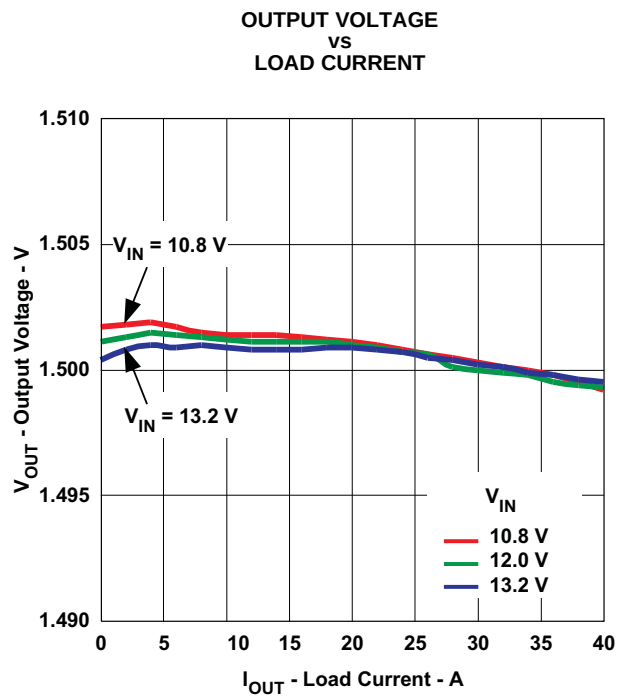
Figure 12. Load Regulation
