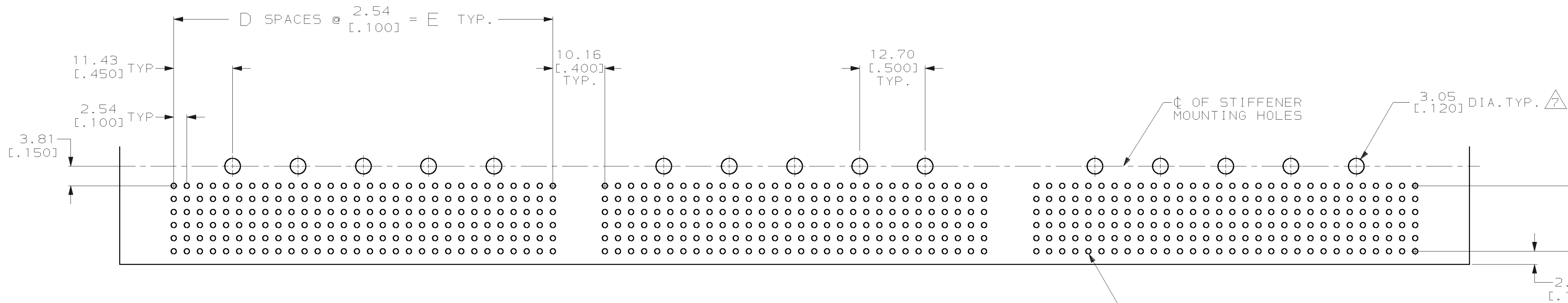
RECOMMENDED P.C. BOARD LAYOUT
