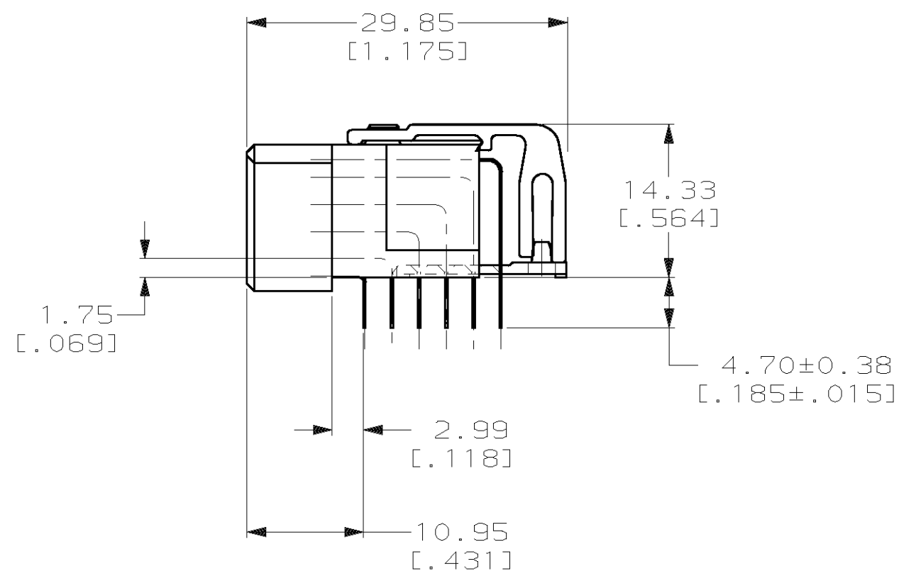
MATING DIMENSIONS REFERENCE
