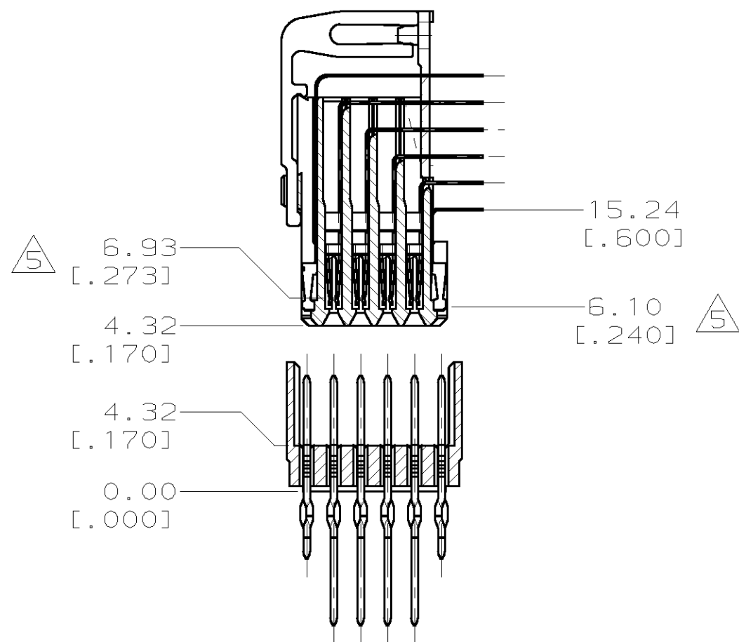
MATING DIMENSIONS REFERENCE
