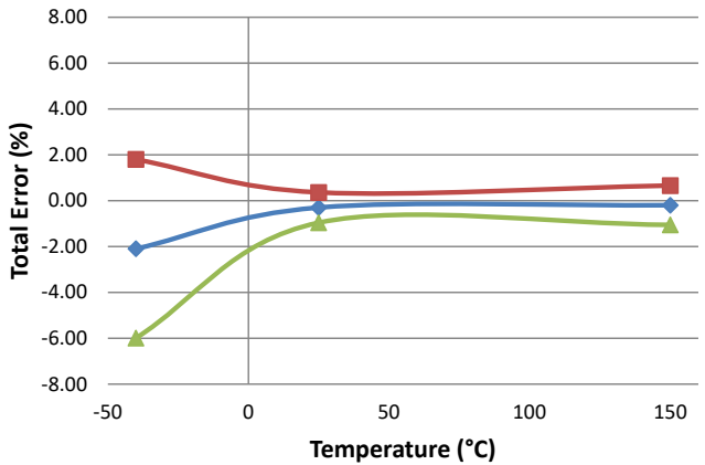
Total Error at I_{PR(max)} vs. Temperature
