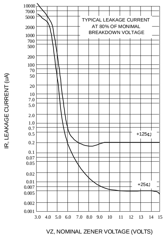
Fig. 8-TYPICAL LEAKAGE CURRENT
