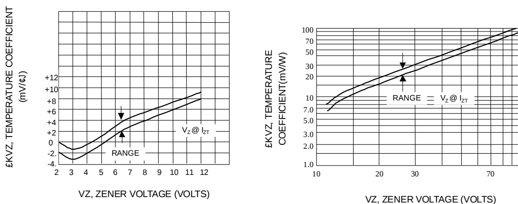
Fig. 2-TEMPERATURE COEFFICIENTS
