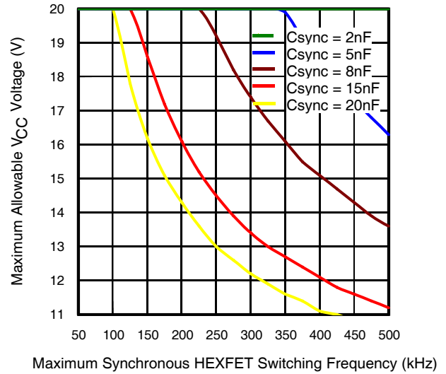
Fig 14. Max V_{CC} Voltage vs. Synchronous Rectifier Switching Freq, T_J = 125^\circ\text{C} , T_{IC} = 85^\circ\text{C} , external R_G = 6\Omega , 1\Omega HEXFET Gate Resistance included
