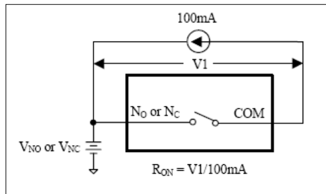
Figure 1. On Resistance
