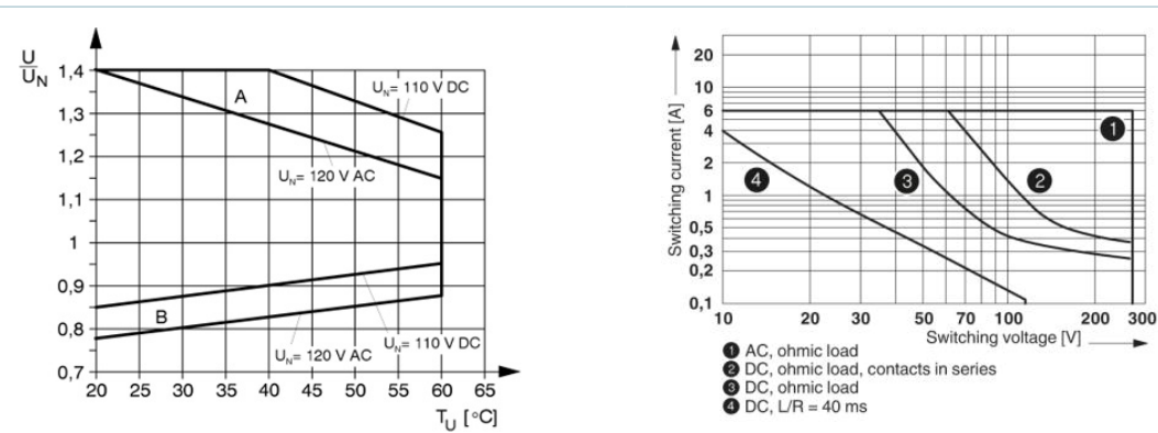
Interrupting rating
