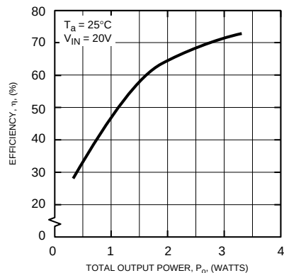
EFFICIENCY CHARACTERISTICS
