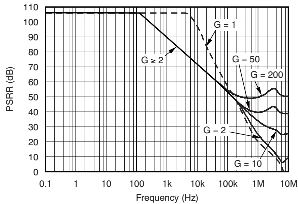
Figure 45. Power-Supply Rejection Ratio vs Frequency
