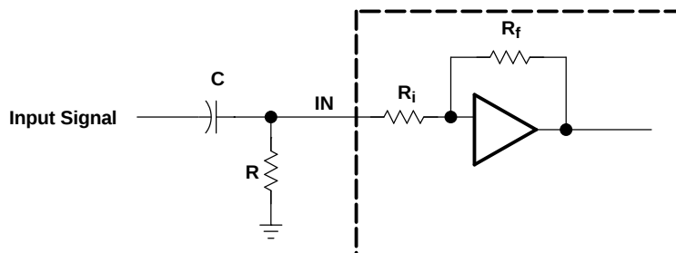
Figure 33. Resistor on Input for Cut-Off Frequency
