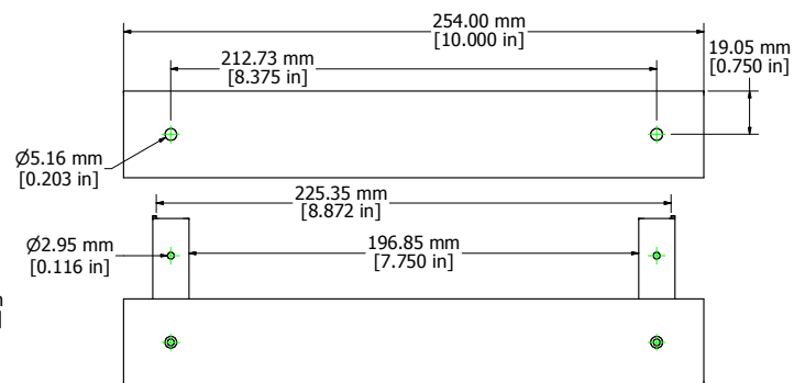
ASSEMBLY - SIDE VIEW (OPEN)
