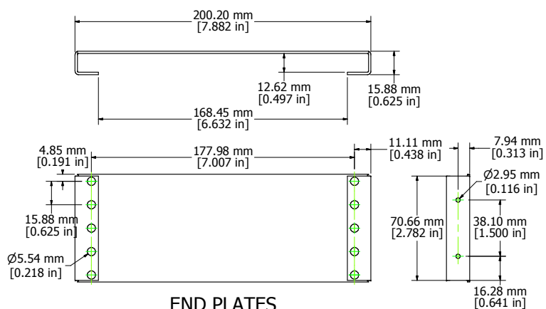
END PLATES
