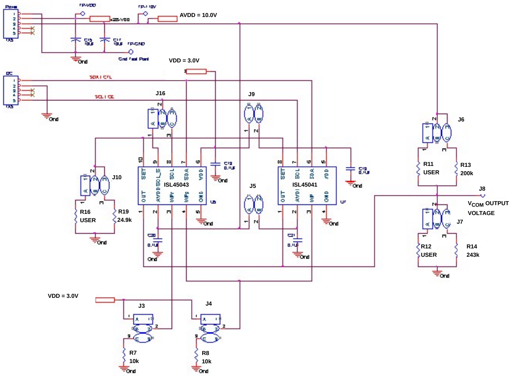
FIGURE 7. ISL45041EVAL1Z SCHEMATIC
