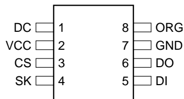
8-Pin SOIC Rotated (R) (1K JEDEC Only)
