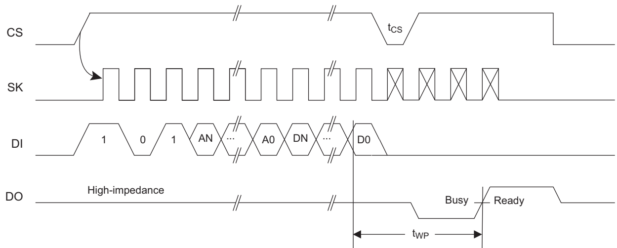
Figure 6-5. WRITE Timing
