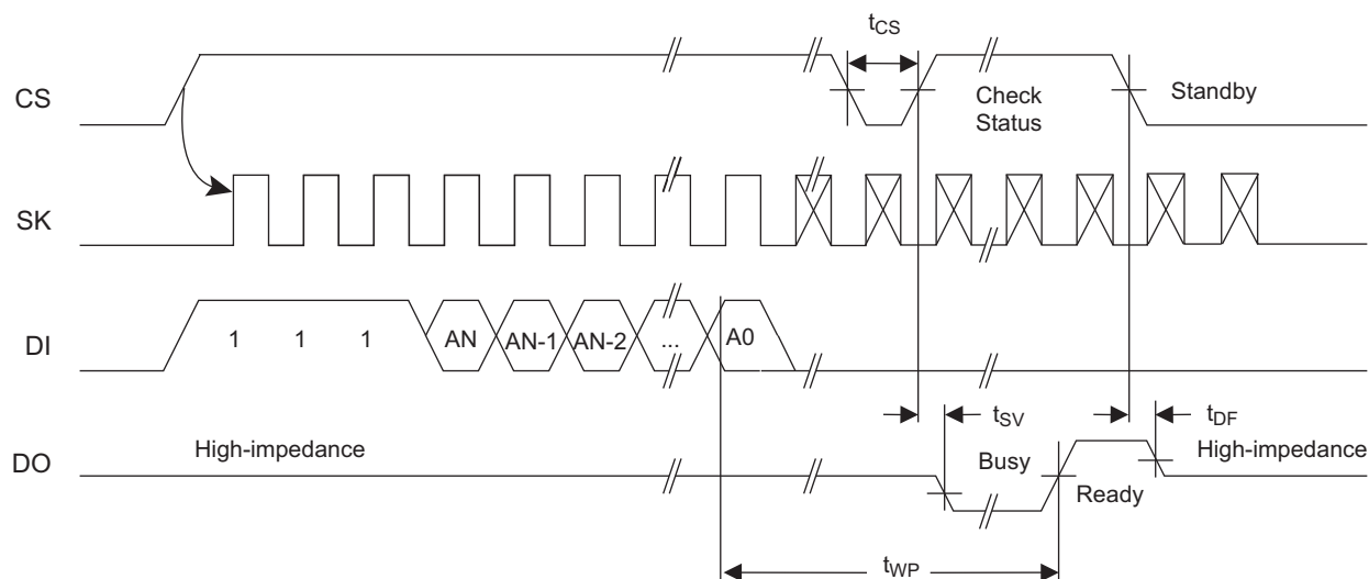
Figure 6-2. ERASE Timing
