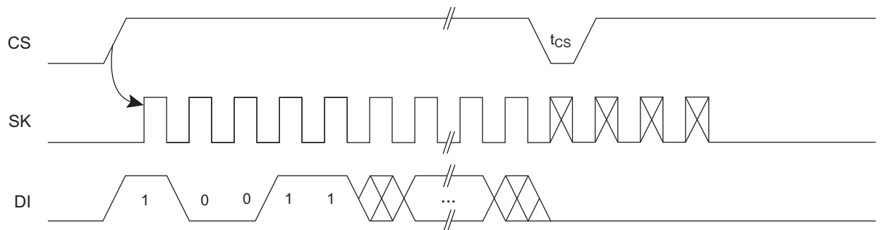
Figure 6-4. EWEN Timing
