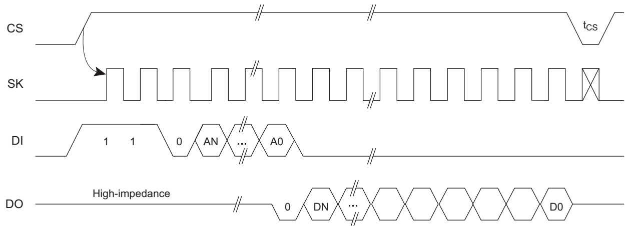
Figure 6-3. READ Timing
