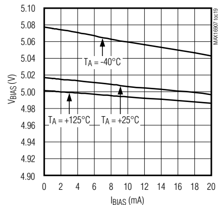
BIAS LOAD REGULATION (5V/2.2MHz)
