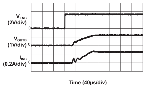
Soft Start
