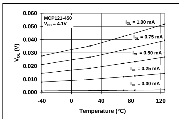
FIGURE 2-21: V_{OL} vs. Temperature (MCP121-450 @ V_{DD} = 4.1\text{V} ).
