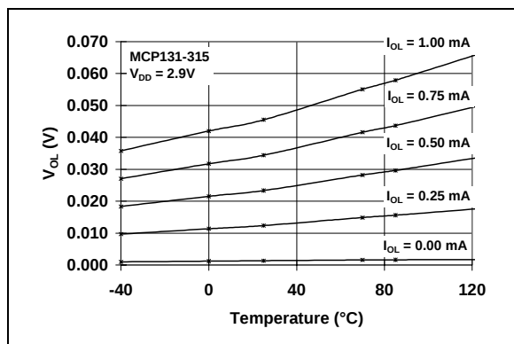
FIGURE 2-20: V_{OL} vs. Temperature (MCP131-315 @ V_{DD} = 2.9\text{V} ).
