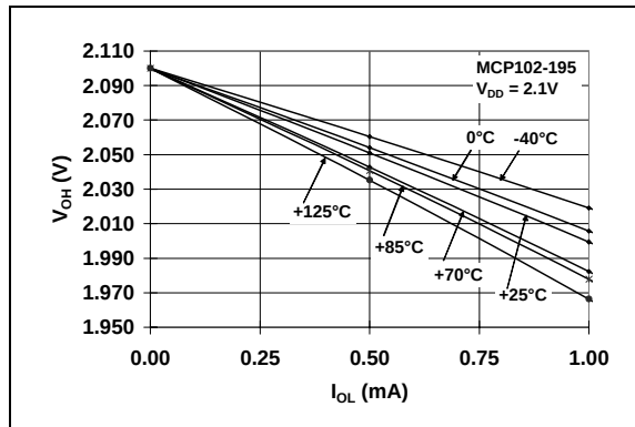
FIGURE 2-22: V_{OH} vs. I_{OL} (MCP102-195 @ V_{DD} = 2.1\text{V} ).
