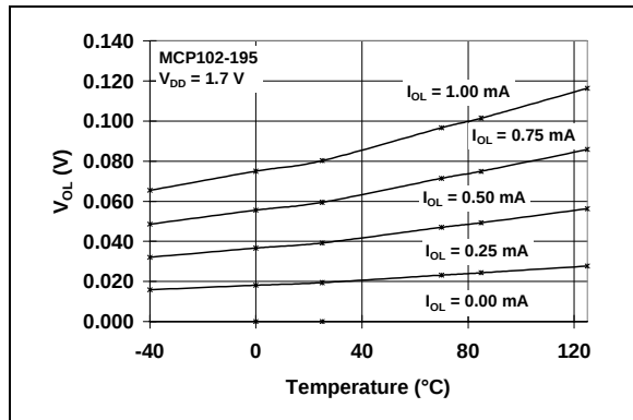
FIGURE 2-19: V_{OL} vs. Temperature (MCP102-195 @ V_{DD} = 1.7\text{V} ).
